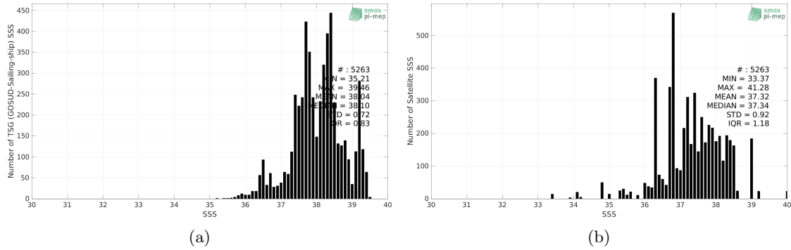
Figure 2: Histograms of SSS from TSG (GOSUD-Sailing-ship) (a) and SMAP SSS L3 v5.0 - Monthly (JPL) (b) considering all match-up pairs per bins of 0.1 over the Mediterranean Sea Pi-MEP region and for the full satellite product period.
