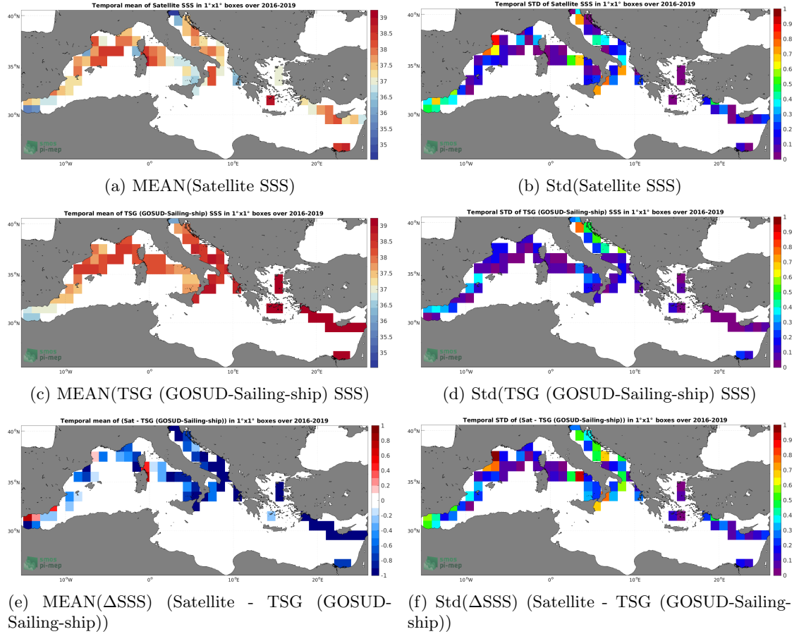
Figure 6: Temporal mean (left) and Std (right) of SSS from SMAP SSS L3 v5.0 - Monthly (JPL) (top), TSG (GOSUD-Sailing-ship) (middle), and of \Delta\text{SSS} (Satellite - TSG (GOSUD-Sailing-ship)). Only match-up pairs are used to generate these maps.
