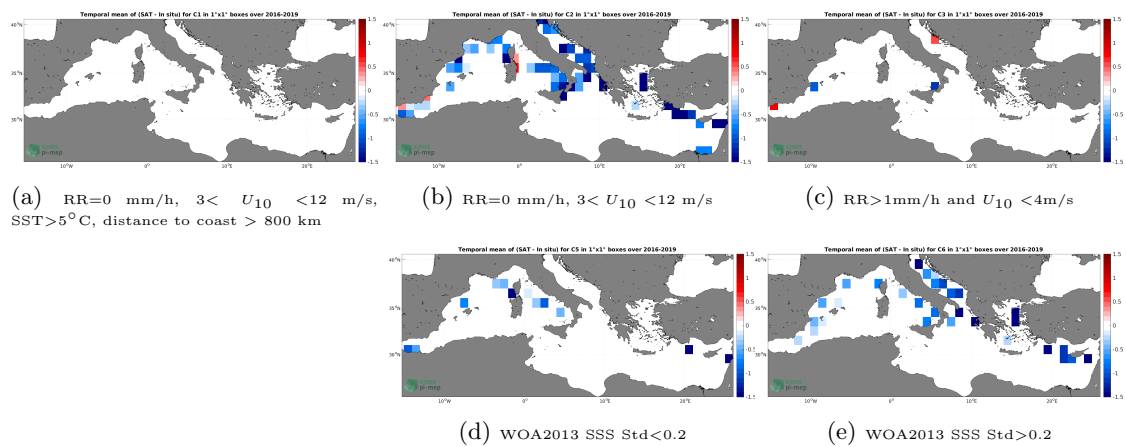
Figure 12: Temporal mean gridded over spatial boxes of size 1^\circ \times 1^\circ of \Delta\text{SSS} (SMAP SSS L3 v5.0 - Monthly (JPL) - TSG (GOSUD-Sailing-ship)) for 5 different subdatasets corresponding to:RR=0 mm/h, 3 < U_{10} < 12 m/s, SST>5°C, distance to coast > 800 km (a), RR=0 mm/h, 3 < U_{10} < 12 m/s (b), RR>1mm/h and U_{10} < 4 m/s (c), WOA2013 SSS Std<0.2 (d), WOA2013 SSS Std>0.2 (e).
