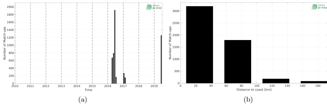
Figure 1: Number of match-ups between TSG (GOSUD-Sailing-ship) and SMAP SSS L3 v5.0 - Monthly (JPL) SSS as a function of time (a) and as function of the distance to coast (b) over the Mediterranean Sea Pi-MEP region and for the full satellite product period.
