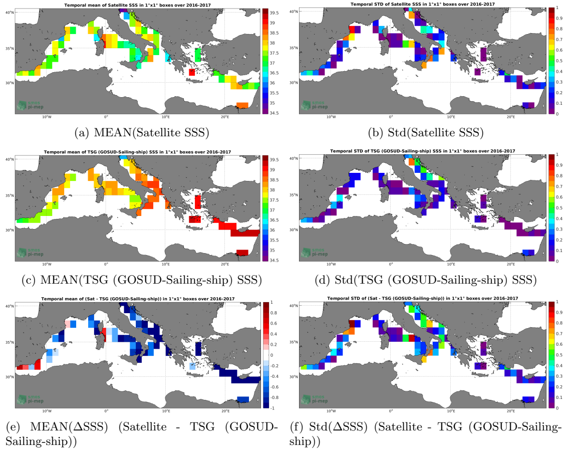
Figure 6: Temporal mean (left) and Std (right) of SSS from SMAP SSS L3 v5.0 - Monthly (JPL) (top), TSG (GOSUD-Sailing-ship) (middle), and of \Delta SSS (Satellite - TSG (GOSUD-Sailing-ship)). Only match-up pairs are used to generate these maps.
