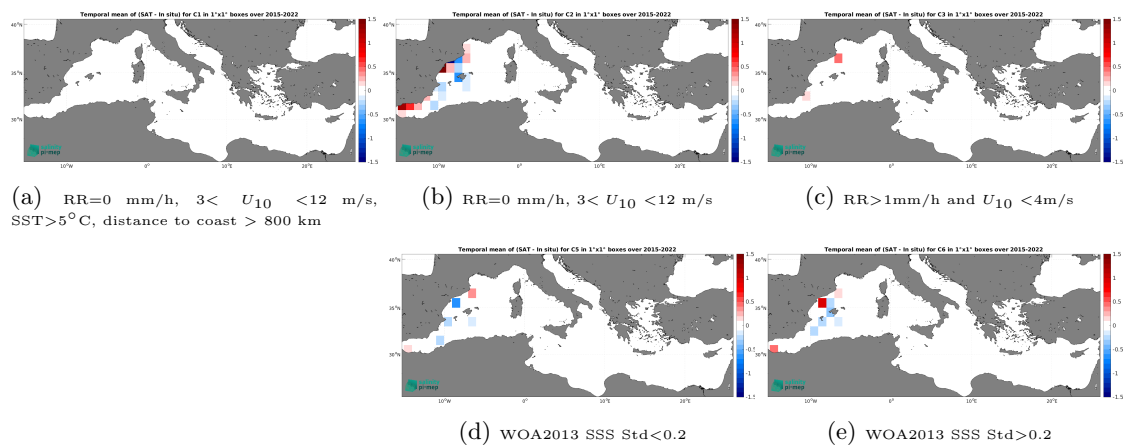
Figure 14: Temporal mean gridded over spatial boxes of size 1^\circ \times 1^\circ of \Delta\text{SSS} (SMAP SSS L3 v5.0 - Monthly (JPL) - TSG (CSIC-UTM)) for 5 different subdatasets corresponding to:RR=0 mm/h, 3 < U_{10} < 12 m/s, SST>5°C, distance to coast > 800 km (a), RR=0 mm/h, 3 < U_{10} < 12 m/s (b), RR>1mm/h and U_{10} < 4 m/s (c), WOA2013 SSS Std<0.2 (d), WOA2013 SSS Std>0.2 (e).
