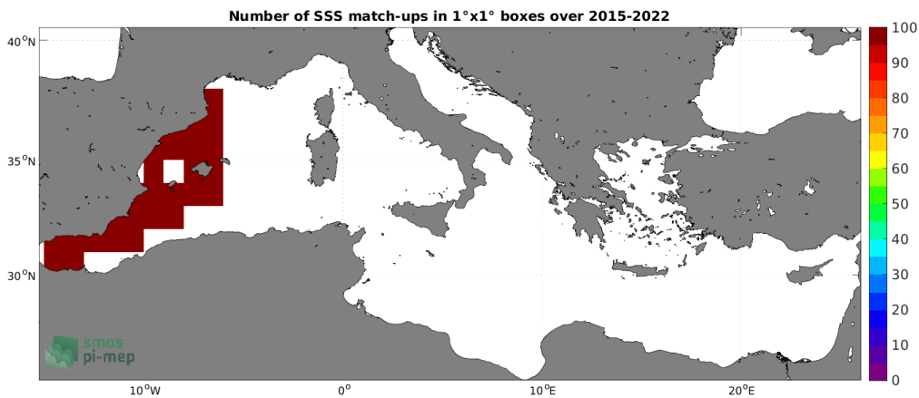
Figure 4: Number of SSS match-ups between TSG (CSIC-UTM) SSS and the SMAP SSS L3 v5.0 - Monthly (JPL) SSS product for the Mediterranean Sea Pi-MEP region over 1^\circ \times 1^\circ boxes and for the full satellite product period.
