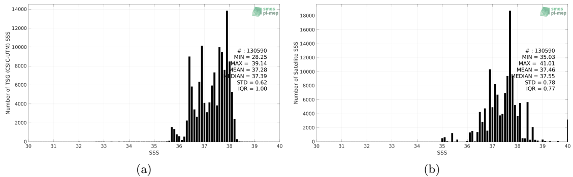
Figure 2: Histograms of SSS from TSG (CSIC-UTM) (a) and SMAP SSS L3 v5.0 - Monthly (JPL) (b) considering all match-up pairs per bins of 0.1 over the Mediterranean Sea Pi-MEP region and for the full satellite product period.
