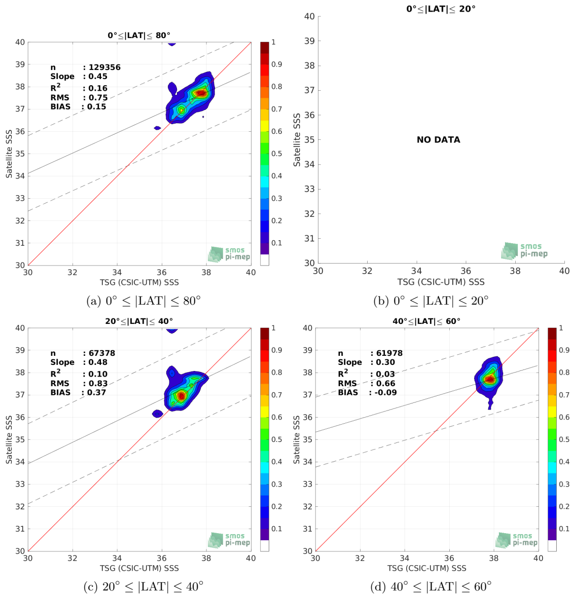
Figure 9: Contour maps of the concentration of SMAP SSS L3 v5.0 - Monthly (JPL) SSS (y-axis) versus TSG (CSIC-UTM) SSS (x-axis) at match-up pairs for different latitude bands. For each plot, the red line shows x=y . The black thin and dashed lines indicate a linear fit through the data cloud and the \pm 95\% confidence levels, respectively. The number match-up pairs n , the slope and R^2 coefficient of the linear fit, the root mean square (RMS) and the mean bias between satellite and in situ data are indicated for each latitude band in each plots.
