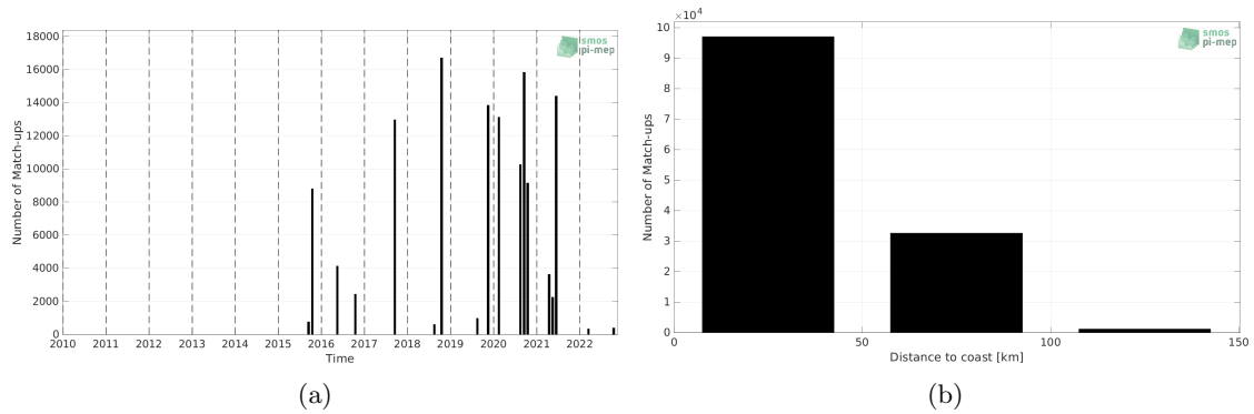
Figure 1: Number of match-ups between TSG (CSIC-UTM) and SMAP SSS L3 v5.0 - Monthly (JPL) SSS as a function of time (a) and as function of the distance to coast (b) over the Mediterranean Sea Pi-MEP region and for the full satellite product period.
