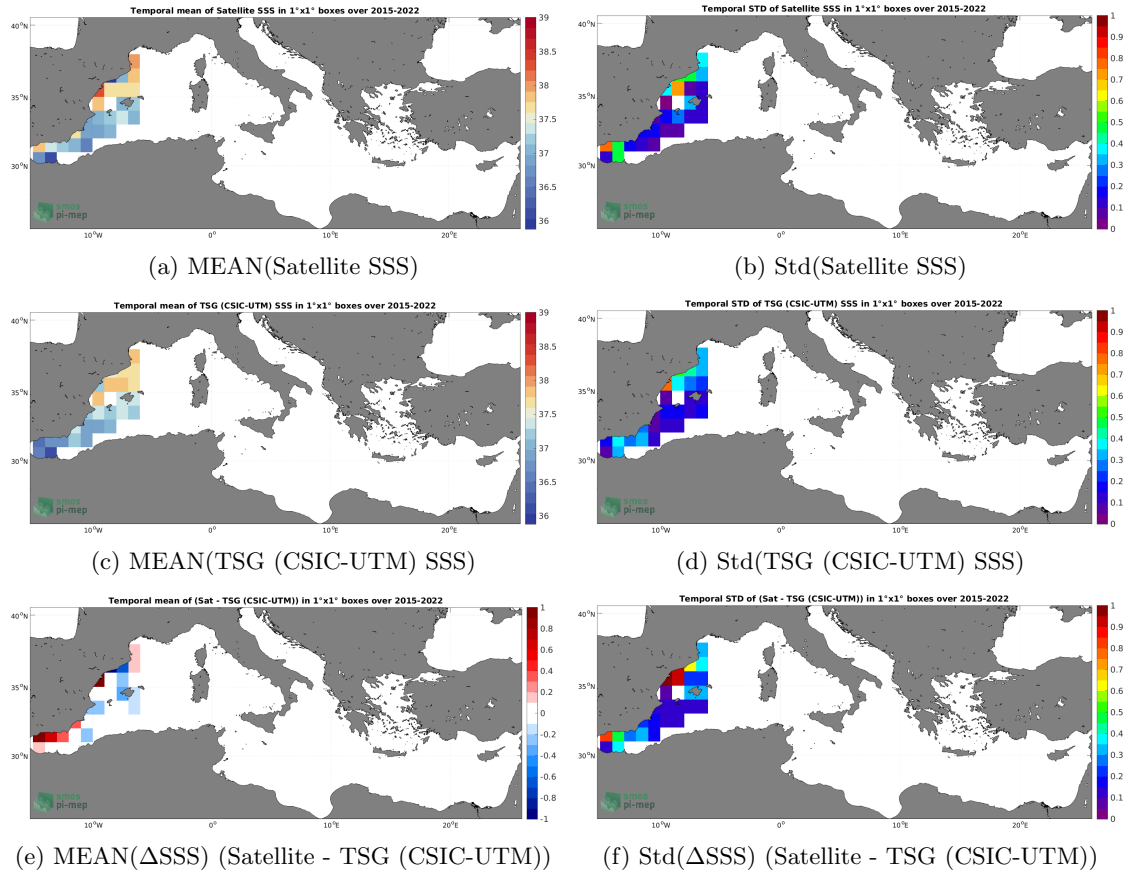
Figure 6: Temporal mean (left) and Std (right) of SSS from SMAP SSS L3 v5.0 - Monthly (JPL) (top), TSG (CSIC-UTM) (middle), and of \Delta SSS (Satellite - TSG (CSIC-UTM)). Only match-up pairs are used to generate these maps.
