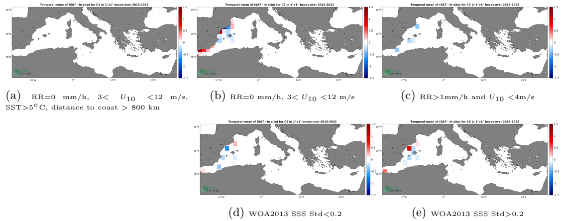
Figure 12: Temporal mean gridded over spatial boxes of size 1^\circ \times 1^\circ of \Delta SSS (SMAP SSS L3 v5.0 - Monthly (JPL) - TSG (CSIC-UTM)) for 5 different subdatasets corresponding to:RR=0 mm/h, 3 < U_{10} < 12 m/s, SST >5^\circ\text{C} , distance to coast > 800 km (a), RR=0 mm/h, 3 < U_{10} < 12 m/s (b), RR >1 mm/h and U_{10} < 4 m/s (c), WOA2013 SSS Std <0.2 (d), WOA2013 SSS Std >0.2 (e).
