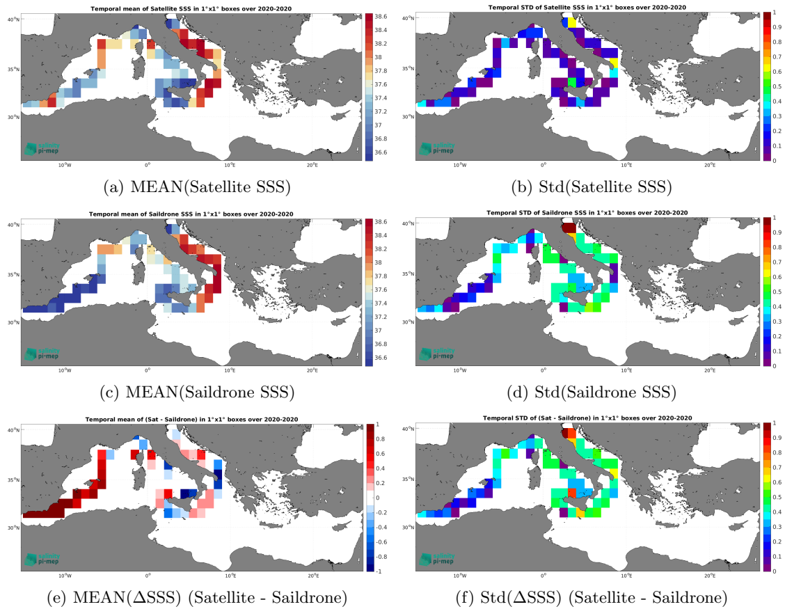
Figure 7: Temporal mean (left) and Std (right) of SSS from SMAP SSS L3 v5.0 - Monthly (JPL) (top), Saildrone (middle), and of \Delta SSS (Satellite - Saildrone). Only match-up pairs are used to generate these maps.
