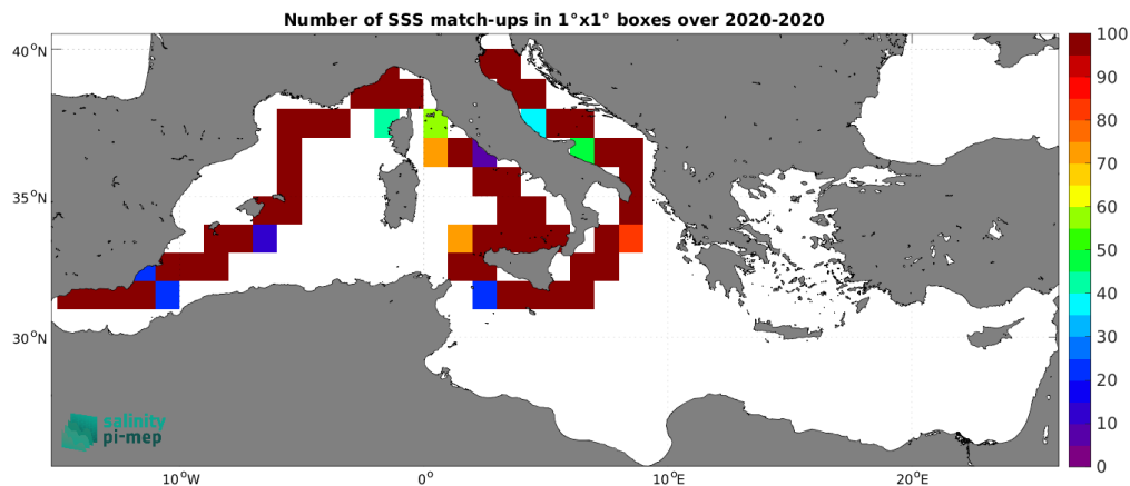
Figure 5: Number of SSS match-ups between Saildrone SSS and the SMAP SSS L3 v5.0 - Monthly (JPL) SSS product for the Mediterranean Sea Pi-MEP region over 1^\circ \times 1^\circ boxes and for the full satellite product period.
