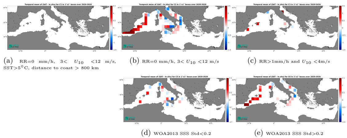
Figure 14: Temporal mean gridded over spatial boxes of size 1^\circ \times 1^\circ of \Delta SSS (SMAP SSS L3 v5.0 - Monthly (JPL) - Saildrone) for 5 different subdatasets corresponding to:RR=0 mm/h, 3 < U_{10} < 12 m/s, SST>5°C, distance to coast > 800 km (a), RR=0 mm/h, 3 < U_{10} < 12 m/s (b), RR>1mm/h and U_{10} < 4 m/s (c), WOA2013 SSS Std<0.2 (d), WOA2013 SSS Std>0.2 (e).
