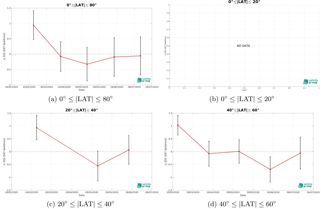
Figure 11: Monthly median (red curves) of \Delta\text{SSS} (Satellite - Sairdrone) and \pm 1 Std (black vertical thick bars) as function of time for all the collected Pi-MEP match-up pairs estimated over the Mediterranean Sea Pi-MEP region and for the full satellite product period are shown for different latitude bands: (a) 80^{\circ}\text{S}-80^{\circ}\text{N} , (b) 20^{\circ}\text{S}-20^{\circ}\text{N} , (c) 40^{\circ}\text{S}-20^{\circ}\text{S} and 20^{\circ}\text{N}-40^{\circ}\text{N} and (d) 60^{\circ}\text{S}-40^{\circ}\text{S} and 40^{\circ}\text{N}-60^{\circ}\text{N} .
