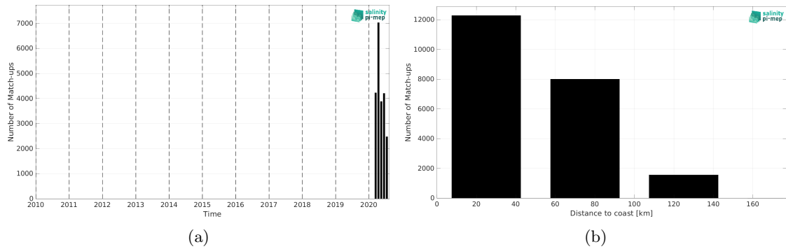
Figure 2: Number of match-ups between Sairdrone and SMAP SSS L3 v5.0 - Monthly (JPL) SSS as a function of time (a) and as function of the distance to coast (b) over the Mediterranean Sea Pi-MEP region and for the full satellite product period.
