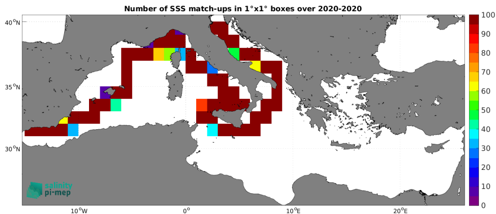
Figure 4: Number of SSS match-ups between Saildrone SSS and the SMAP SSS L3 v5.0 - Monthly (JPL) SSS product for the Mediterranean Sea Pi-MEP region over 1^\circ \times 1^\circ boxes and for the full satellite product period.
