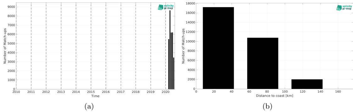
Figure 1: Number of match-ups between Saildrone and SMAP SSS L3 v5.0 - Monthly (JPL) SSS as a function of time (a) and as function of the distance to coast (b) over the Mediterranean Sea Pi-MEP region and for the full satellite product period.
