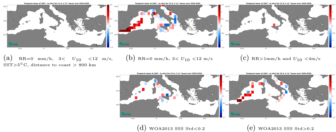
Figure 12: Temporal mean gridded over spatial boxes of size 1^\circ \times 1^\circ of \Delta SSS (SMAP SSS L3 v5.0 - Monthly (JPL) - Saildrone) for 5 different subdatasets corresponding to:RR=0 mm/h, 3 < U_{10} < 12 m/s, SST >5^\circ\text{C} , distance to coast > 800 km (a), RR=0 mm/h, 3 < U_{10} < 12 m/s (b), RR >1 mm/h and U_{10} < 4 m/s (c), WOA2013 SSS Std <0.2 (d), WOA2013 SSS Std >0.2 (e).
