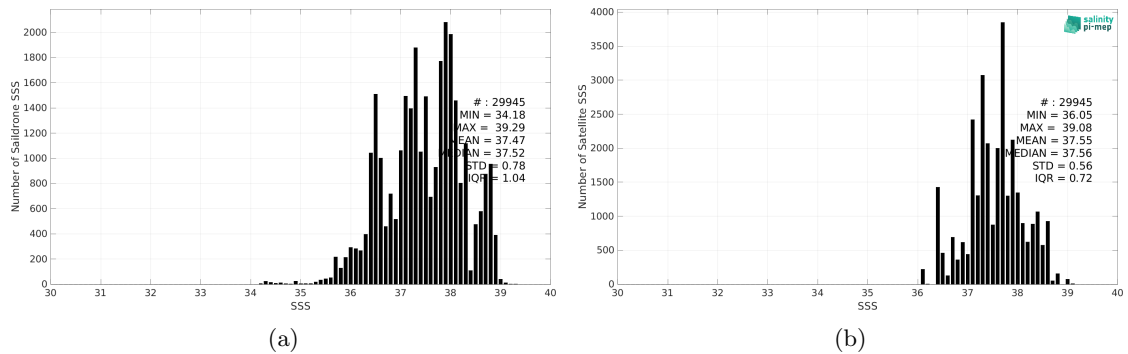
Figure 2: Histograms of SSS from Saildrone (a) and SMAP SSS L3 v5.0 - Monthly (JPL) (b) considering all match-up pairs per bins of 0.1 over the Mediterranean Sea Pi-MEP region and for the full satellite product period.
