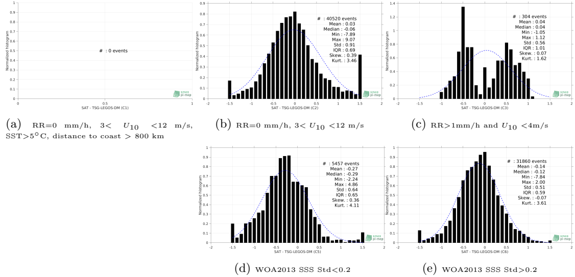
Figure 13: Normalized histogram of \Delta SSS (SMAP-L3-JPL-V4.3-8DAY-RUNNING-60KM - TSG-LEGOS-DM) for 5 different subdatasets corresponding to: RR=0 mm/h, 3 < U_{10} < 12 m/s, SST>5°C, distance to coast > 800 km (a), RR=0 mm/h, 3 < U_{10} < 12 m/s (b), RR>1mm/h and U_{10} < 4 m/s (c), WOA2013 SSS Std<0.2 (d), WOA2013 SSS Std>0.2 (e).
