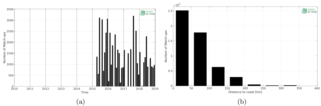
Figure 1: Number of match-ups between TSG-LEGOS-DM and SMAP-L3-JPL-V4.3-8DAY-RUNNING-60KM SSS as a function of time (a) and as function of the distance to coast (b) over the Mediterranean Sea Pi-MEP region and for the full satellite product period.
