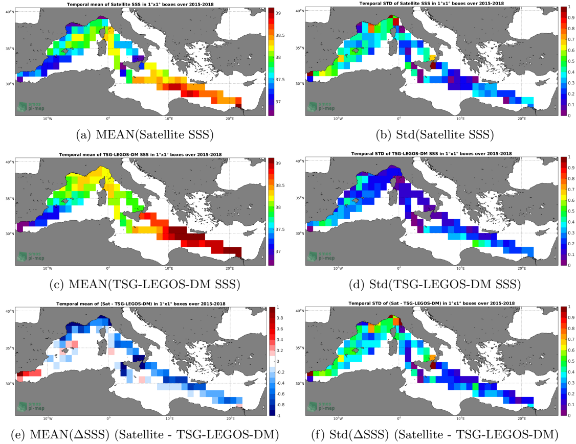
Figure 6: Temporal mean (left) and Std (right) of SSS from SMAP-L3-JPL-V4.3-8DAY-RUNNING-60KM (top), TSG-LEGOS-DM (middle), and of \Delta SSS (Satellite - TSG-LEGOS-DM). Only match-up pairs are used to generate these maps.
