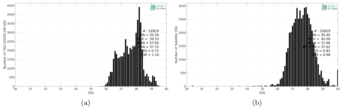
Figure 2: Histograms of SSS from TSG-LEGOS-DM (a) and SMAP-L3-JPL-V4.3-8DAY-RUNNING-60KM (b) considering all match-up pairs per bins of 0.1 over the Mediterranean Sea Pi-MEP region and for the full satellite product period.
