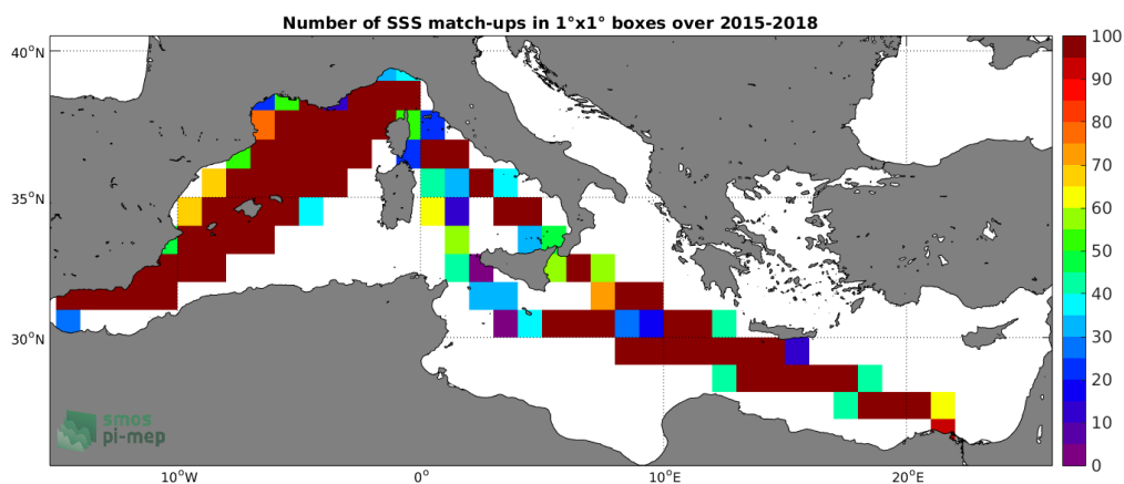
Figure 4: Number of SSS match-ups between TSG-LEGOS-DM SSS and the SMAP-L3-JPL-V4.3-8DAY-RUNNING-60KM SSS product for the Mediterranean Sea Pi-MEP region over 1^\circ \times 1^\circ boxes and for the full satellite product period.
