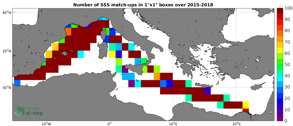
Figure 4: Number of SSS match-ups between TSG-LEGOS-DM SSS and the SMAP-L3-JPL-V4.3-8DAY-RUNNING-60KM SSS product for the Mediterranean Sea Pi-MEP region over 1°x1° boxes and for the full satellite product period.
