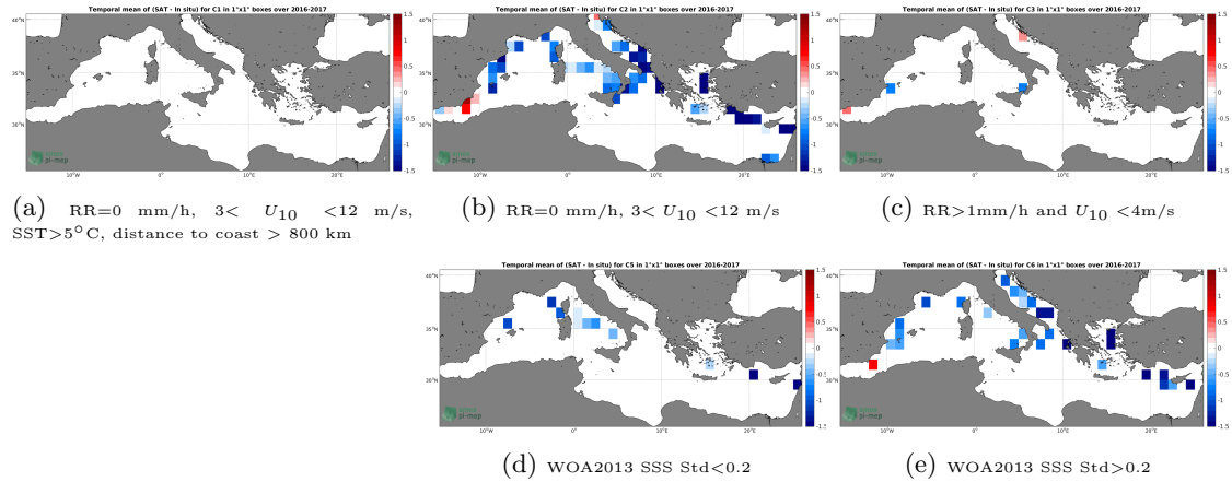
Figure 12: Temporal mean gridded over spatial boxes of size 1^{\circ}\times 1^{\circ} of \Delta SSS (SMAP-L3-JPL-V4.3-8DAY-RUNNING-60KM - TSG-GOSUD-Sailing-ship) for 5 different subdatasets corresponding to:RR=0 mm/h, 3 < U_{10} < 12 m/s, SST >5^{\circ}\text{C} , distance to coast > 800 km (a), RR=0 mm/h, 3 < U_{10} < 12 m/s (b), RR >1 mm/h and U_{10} < 4 m/s (c), WOA2013 SSS Std <0.2 (d), WOA2013 SSS Std >0.2 (e).
