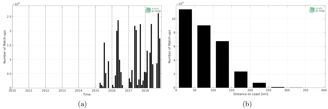
Figure 1: Number of match-ups between TSG-GOSUD-Research-vessel and SMAP-L3-JPL-V4.3-8DAY-RUNNING-60KM SSS as a function of time (a) and as function of the distance to coast (b) over the Mediterranean Sea Pi-MEP region and for the full satellite product period.
