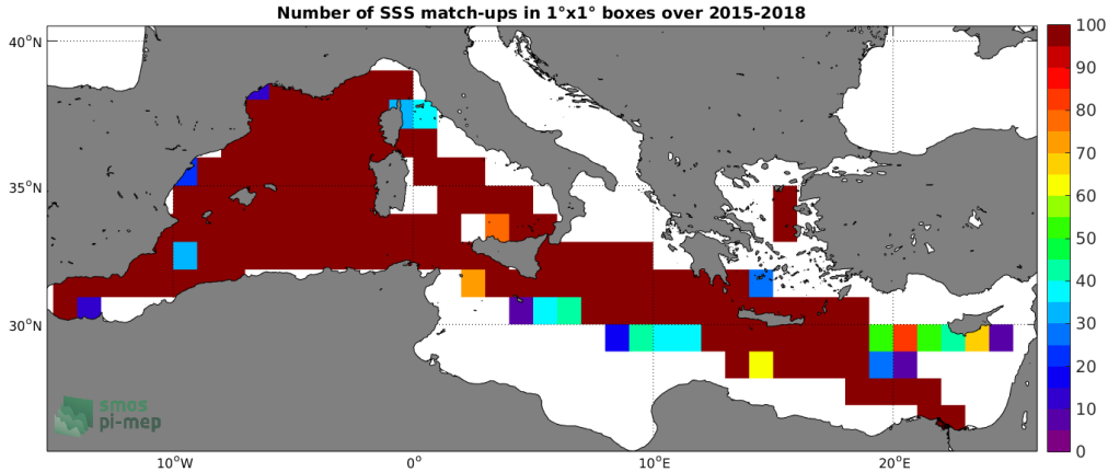
Figure 4: Number of SSS match-ups between TSG-GOSUD-Research-vessel SSS and the SMAP-L3-JPL-V4.3-8DAY-RUNNING-60KM SSS product for the Mediterranean Sea Pi-MEP region over 1°x1° boxes and for the full satellite product period.
