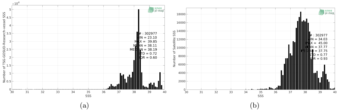
Figure 2: Histograms of SSS from TSG-GOSUD-Research-vessel (a) and SMAP-L3-JPL-V4.3-8DAY-RUNNING-60KM (b) considering all match-up pairs per bins of 0.1 over the Mediterranean Sea Pi-MEP region and for the full satellite product period.
