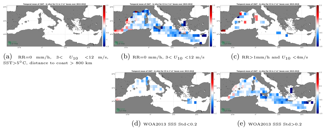
Figure 12: Temporal mean gridded over spatial boxes of size 1^\circ \times 1^\circ of \Delta SSS (SMAP-L3-JPL-V4.3-8DAY-RUNNING-60KM - TSG-GOSUD-Research-vessel) for 5 different subdatasets corresponding to:RR=0 mm/h, 3 < U_{10} < 12 m/s, SST >5^\circ\text{C} , distance to coast > 800 km (a), RR=0 mm/h, 3 < U_{10} < 12 m/s (b), RR >1 mm/h and U_{10} < 4 m/s (c), WOA2013 SSS Std <0.2 (d), WOA2013 SSS Std >0.2 (e).
