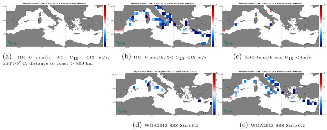
Figure 12: Temporal mean gridded over spatial boxes of size 1^\circ \times 1^\circ of \Delta SSS (SMAP-L3-JPL-V4.3-MONTHLY-60KM - TSG-GOSUD-Sailing-ship) for 5 different subdatasets corresponding to:RR=0 mm/h, 3 < U_{10} < 12 m/s, SST>5°C, distance to coast > 800 km (a), RR=0 mm/h, 3 < U_{10} < 12 m/s (b), RR>1mm/h and U_{10} < 4 m/s (c), WOA2013 SSS Std<0.2 (d), WOA2013 SSS Std>0.2 (e).
