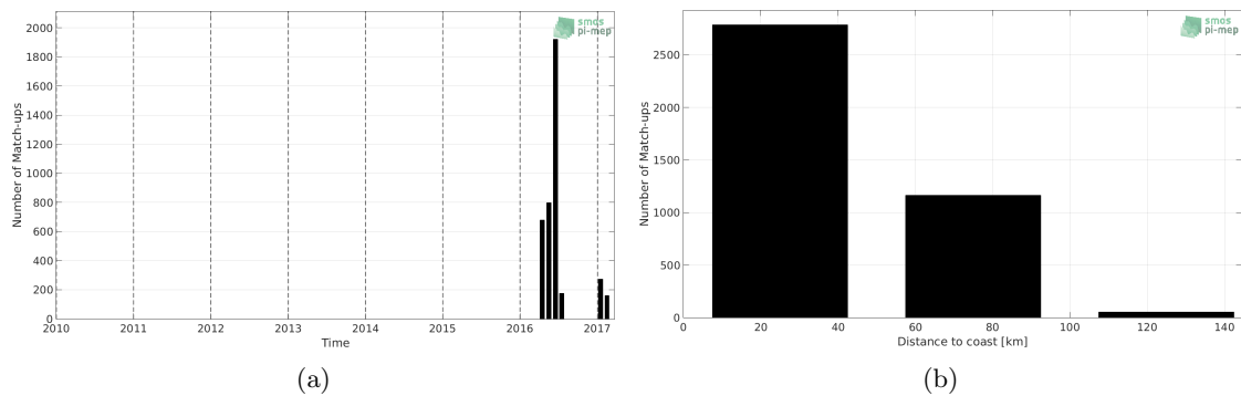
Figure 1: Number of match-ups between TSG-GOSUD-Sailing-ship and SMAP-L3-JPL-V4.3-MONTHLY-60KM SSS as a function of time (a) and as function of the distance to coast (b) over the Mediterranean Sea Pi-MEP region and for the full satellite product period.
