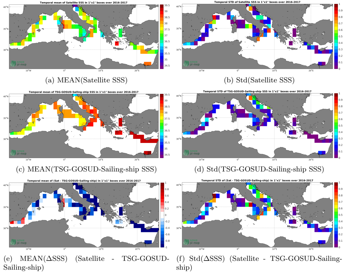
Figure 6: Temporal mean (left) and Std (right) of SSS from SMAP-L3-JPL-V4.3-MONTHLY-60KM (top), TSG-GOSUD-Sailing-ship (middle), and of \Delta SSS (Satellite - TSG-GOSUD-Sailing-ship). Only match-up pairs are used to generate these maps.
