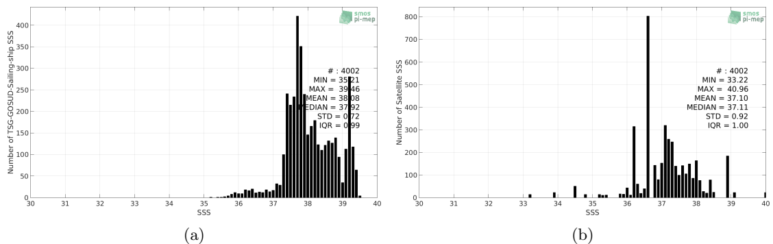
Figure 2: Histograms of SSS from TSG-GOSUD-Sailing-ship (a) and SMAP-L3-JPL-V4.3-MONTHLY-60KM (b) considering all match-up pairs per bins of 0.1 over the Mediterranean Sea Pi-MEP region and for the full satellite product period.
