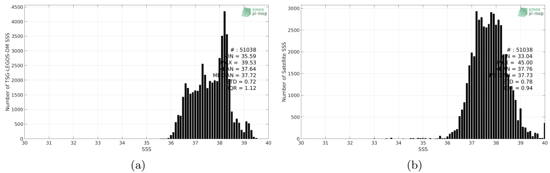
Figure 2: Histograms of SSS from TSG-LEGOS-DM (a) and SMAP-L3-JPL-V4.2-8DAY-RUNNING-60KM (b) considering all match-up pairs per bins of 0.1 over the Mediterranean Sea Pi-MEP region and for the full satellite product period.
