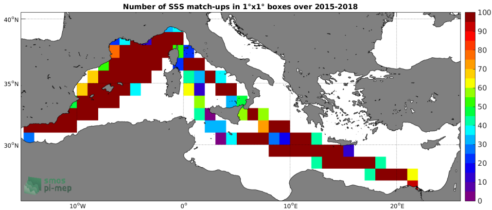
Figure 4: Number of SSS match-ups between TSG-LEGOS-DM SSS and the SMAP-L3-JPL-V4.2-8DAY-RUNNING-60KM SSS product for the Mediterranean Sea Pi-MEP region over 1^\circ \times 1^\circ boxes and for the full satellite product period.
