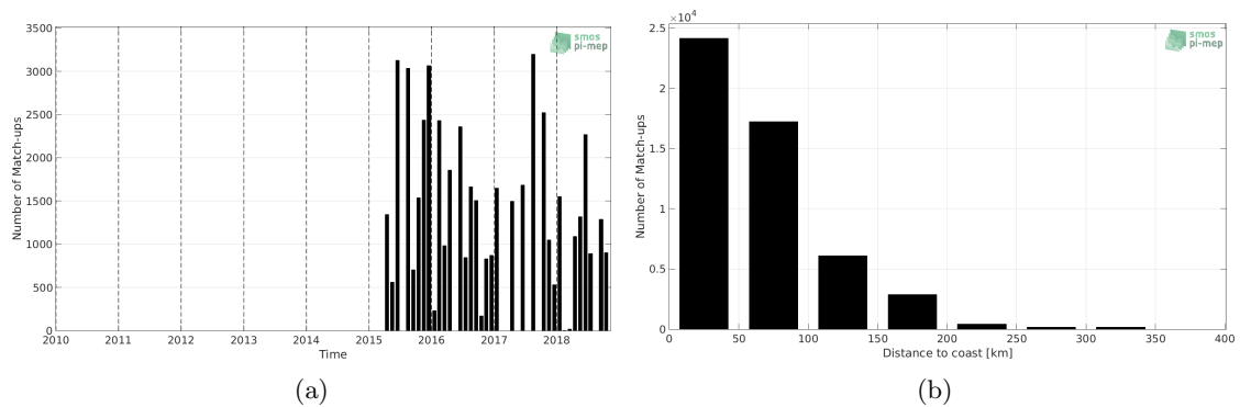
Figure 1: Number of match-ups between TSG-LEGOS-DM and SMAP-L3-JPL-V4.2-8DAY-RUNNING-60KM SSS as a function of time (a) and as function of the distance to coast (b) over the Mediterranean Sea Pi-MEP region and for the full satellite product period.
