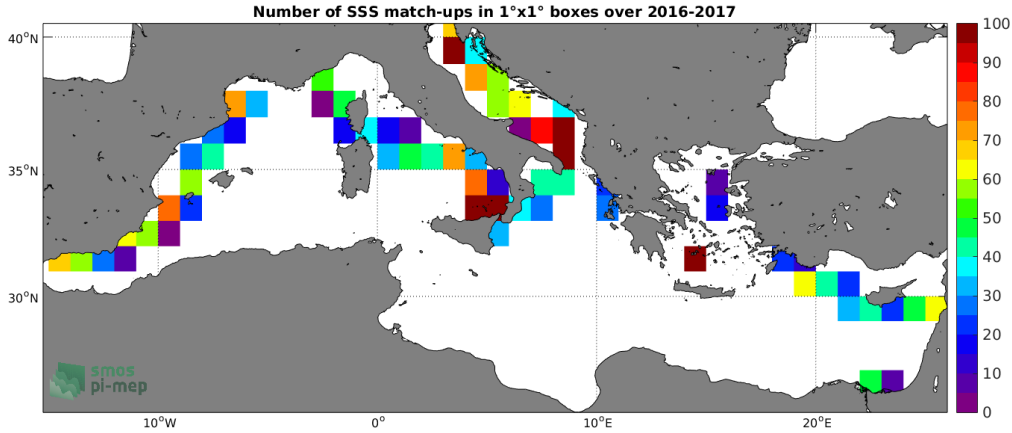
Figure 4: Number of SSS match-ups between TSG-GOSUD-Sailing-ship SSS and the SMAP-L3-JPL-V4.2-8DAY-RUNNING-60KM SSS product for the Mediterranean Sea Pi-MEP region over 1^\circ \times 1^\circ boxes and for the full satellite product period.
