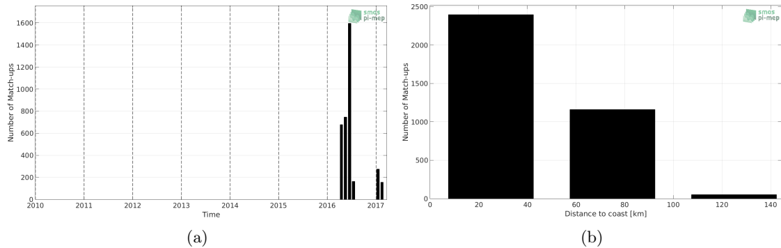
Figure 1: Number of match-ups between TSG-GOSUD-Sailing-ship and SMAP-L3-JPL-V4.2-8DAY-RUNNING-60KM SSS as a function of time (a) and as function of the distance to coast (b) over the Mediterranean Sea Pi-MEP region and for the full satellite product period.
