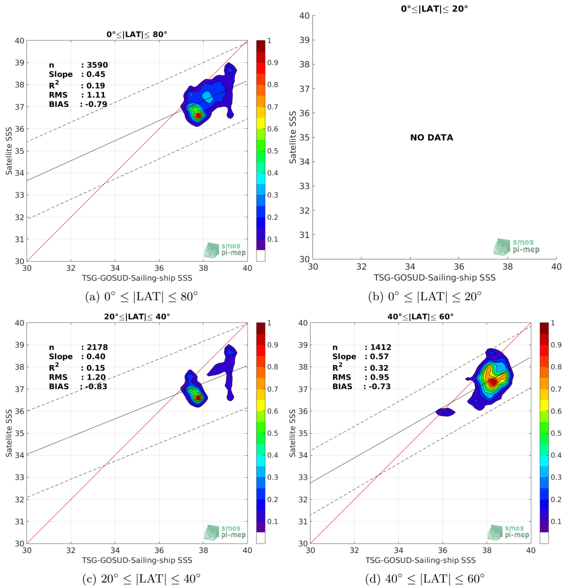
Figure 9: Contour maps of the concentration of SMAP-L3-JPL-V4.2-8DAY-RUNNING-60KM SSS (y-axis) versus TSG-GOSUD-Sailing-ship SSS (x-axis) at match-up pairs for different latitude bands. For each plot, the red line shows x=y . The black thin and dashed lines indicate a linear fit through the data cloud and the \pm 95\% confidence levels, respectively. The number of match-up pairs n , the slope and R^2 coefficient of the linear fit, the root mean square (RMS) and the mean bias between satellite and in situ data are indicated for each latitude band in each plot.
