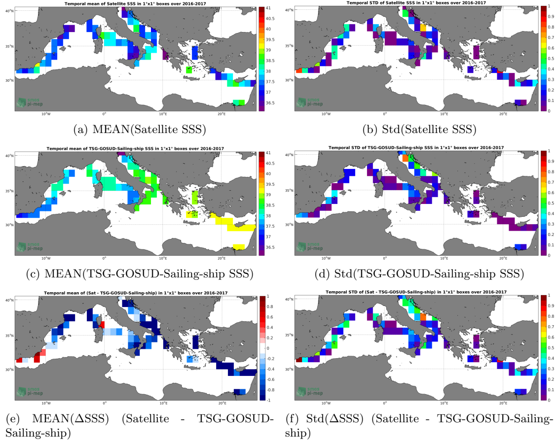
Figure 6: Temporal mean (left) and Std (right) of SSS from SMAP-L3-JPL-V4.2-8DAY-RUNNING-60KM (top), TSG-GOSUD-Sailing-ship (middle), and of \Delta SSS (Satellite - TSG-GOSUD-Sailing-ship). Only match-up pairs are used to generate these maps.
