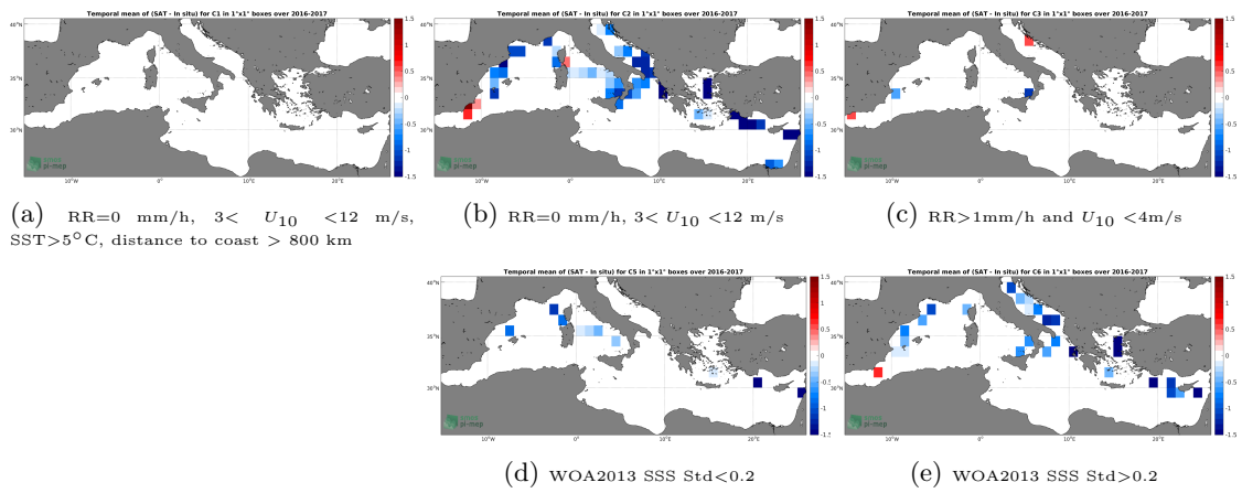
Figure 12: Temporal mean gridded over spatial boxes of size 1^\circ \times 1^\circ of \Delta SSS (SMAP-L3-JPL-V4.2-8DAY-RUNNING-60KM - TSG-GOSUD-Sailing-ship) for 5 different subdatasets corresponding to:RR=0 mm/h, 3 < U_{10} < 12 m/s, SST>5°C, distance to coast > 800 km (a), RR=0 mm/h, 3 < U_{10} < 12 m/s (b), RR>1mm/h and U_{10} < 4 m/s (c), WOA2013 SSS Std<0.2 (d), WOA2013 SSS Std>0.2 (e).
