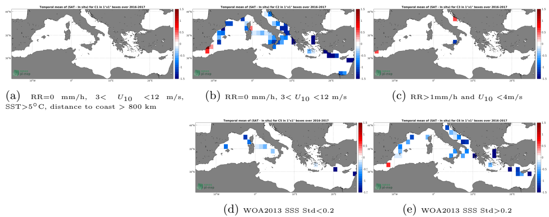
Figure 12: Temporal mean gridded over spatial boxes of size 1^\circ \times 1^\circ of \Delta SSS (SMAP-L3-JPL-V4.2-8DAY-RUNNING-60KM - TSG-GOSUD-Sailing-ship) for 5 different subdatasets corresponding to:RR=0 mm/h, 3 < U_{10} < 12 m/s, SST >5^\circ\text{C} , distance to coast > 800 km (a), RR=0 mm/h, 3 < U_{10} < 12 m/s (b), RR >1 mm/h and U_{10} < 4 m/s (c), WOA2013 SSS Std <0.2 (d), WOA2013 SSS Std >0.2 (e).
