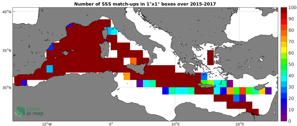
Figure 4: Number of SSS match-ups between TSG-GOSUD-Research-vessel SSS and the SMAP-L3-JPL-V4.2-8DAY-RUNNING-60KM SSS product for the Mediterranean Sea Pi-MEP region over 1^\circ \times 1^\circ boxes and for the full satellite product period.
