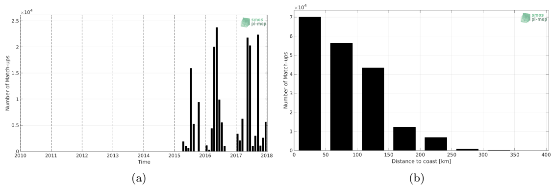
Figure 1: Number of match-ups between TSG-GOSUD-Research-vessel and SMAP-L3-JPL-V4.2-8DAY-RUNNING-60KM SSS as a function of time (a) and as function of the distance to coast (b) over the Mediterranean Sea Pi-MEP region and for the full satellite product period.
