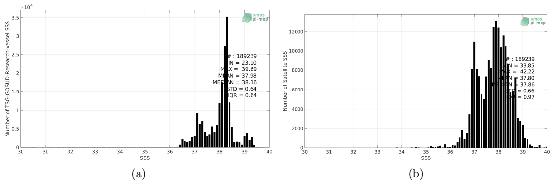
Figure 2: Histograms of SSS from TSG-GOSUD-Research-vessel (a) and SMAP-L3-JPL-V4.2-8DAY-RUNNING-60KM (b) considering all match-up pairs per bins of 0.1 over the Mediterranean Sea Pi-MEP region and for the full satellite product period.
