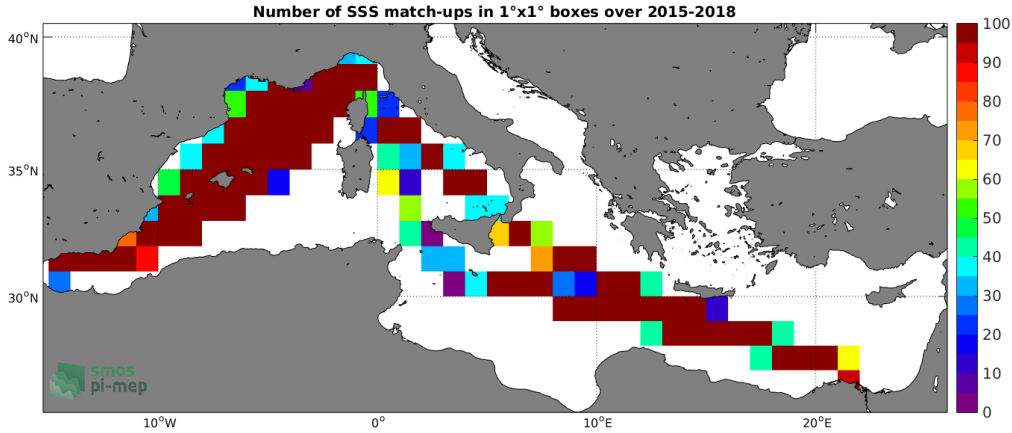
Figure 4: Number of SSS match-ups between TSG-LEGOS-DM SSS and the SMAP-L3-JPL-V4.2-MONTHLY-60KM SSS product for the Mediterranean Sea Pi-MEP region over 1°x1° boxes and for the full satellite product period.
