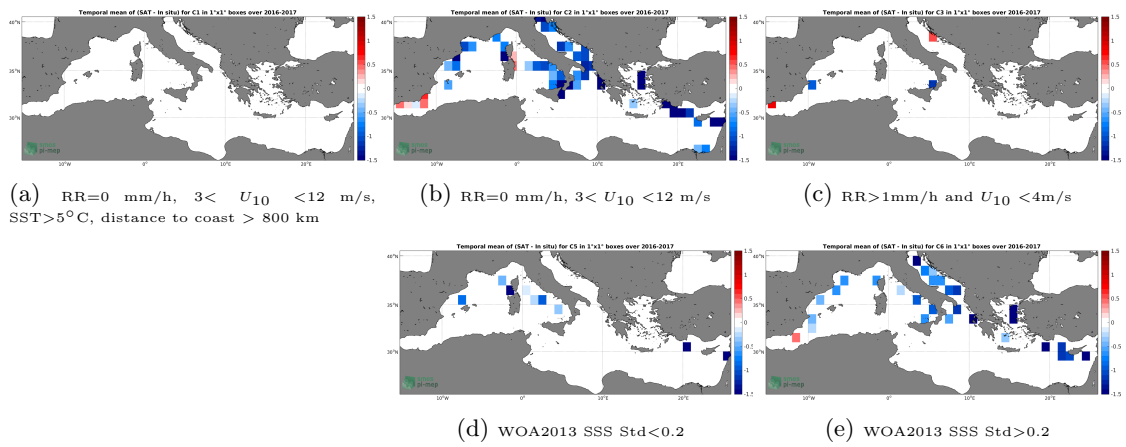
Figure 12: Temporal mean gridded over spatial boxes of size 1^\circ \times 1^\circ of \Delta SSS (SMAP-L3-JPL-V4.2-MONTHLY-60KM - TSG-GOSUD-Sailing-ship) for 5 different subdatasets corresponding to:RR=0 mm/h, 3 < U_{10} < 12 m/s, SST >5^\circ\text{C} , distance to coast > 800 km (a), RR=0 mm/h, 3 < U_{10} < 12 m/s (b), RR >1 mm/h and U_{10} < 4 m/s (c), WOA2013 SSS Std <0.2 (d), WOA2013 SSS Std >0.2 (e).
