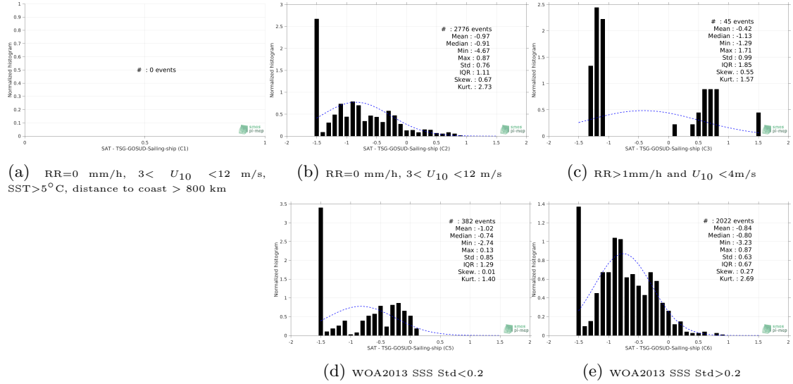
Figure 13: Normalized histogram of \Delta SSS (SMAP-L3-JPL-V4.2-MONTHLY-60KM - TSG-GOSUD-Sailing-ship) for 5 different subdatasets corresponding to: RR=0 mm/h, 3 < U_{10} < 12 m/s, SST > 5°C, distance to coast > 800 km (a), RR=0 mm/h, 3 < U_{10} < 12 m/s (b), RR > 1mm/h and U_{10} < 4 m/s (c), WOA2013 SSS Std < 0.2 (d), WOA2013 SSS Std > 0.2 (e).
