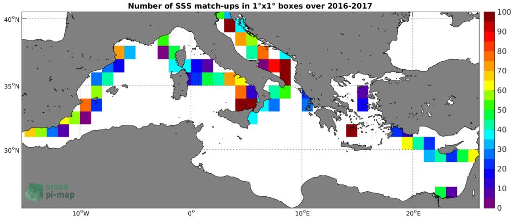
Figure 4: Number of SSS match-ups between TSG-GOSUD-Sailing-ship SSS and the SMAP-L3-JPL-V4.2-MONTHLY-60KM SSS product for the Mediterranean Sea Pi-MEP region over 1^\circ \times 1^\circ boxes and for the full satellite product period.
