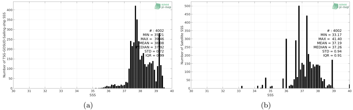
Figure 2: Histograms of SSS from TSG-GOSUD-Sailing-ship (a) and SMAP-L3-JPL-V4.2-MONTHLY-60KM (b) considering all match-up pairs per bins of 0.1 over the Mediterranean Sea Pi-MEP region and for the full satellite product period.
