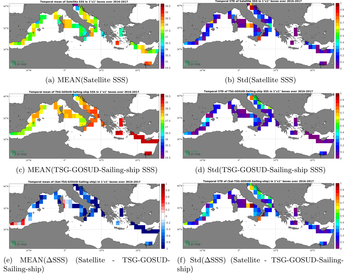
Figure 6: Temporal mean (left) and Std (right) of SSS from SMAP-L3-JPL-V4.2-MONTHLY-60KM (top), TSG-GOSUD-Sailing-ship (middle), and of \Delta SSS (Satellite - TSG-GOSUD-Sailing-ship). Only match-up pairs are used to generate these maps.
