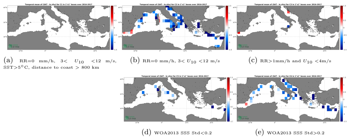
Figure 12: Temporal mean gridded over spatial boxes of size 1^\circ \times 1^\circ of \Delta SSS (SMAP-L3-JPL-V4.2-MONTHLY-60KM - TSG-GOSUD-Sailing-ship) for 5 different subdatasets corresponding to:RR=0 mm/h, 3 < U_{10} < 12 m/s, SST >5^\circ C, distance to coast > 800 km (a), RR=0 mm/h, 3 < U_{10} < 12 m/s (b), RR >1 mm/h and U_{10} < 4 m/s (c), WOA2013 SSS Std <0.2 (d), WOA2013 SSS Std >0.2 (e).
