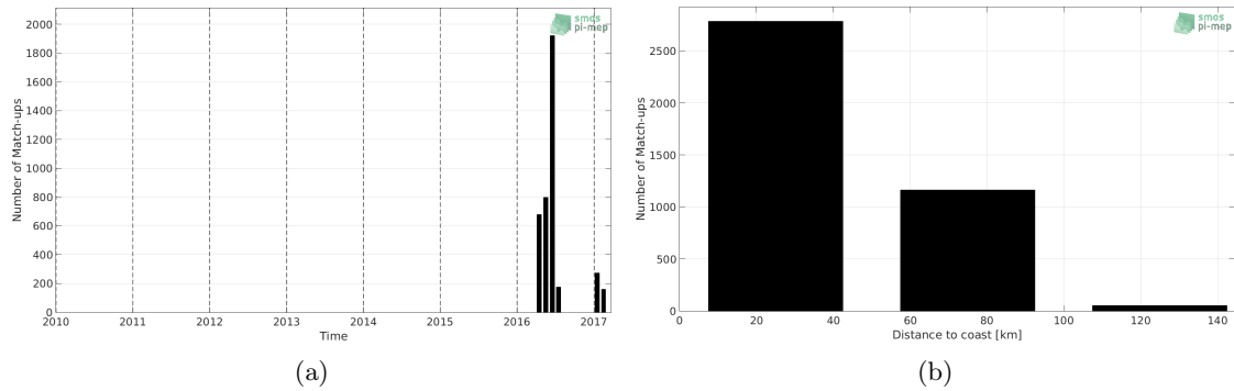
Figure 1: Number of match-ups between TSG-GOSUD-Sailing-ship and SMAP-L3-JPL-V4.2-MONTHLY-60KM SSS as a function of time (a) and as function of the distance to coast (b) over the Mediterranean Sea Pi-MEP region and for the full satellite product period.
