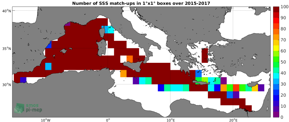
Figure 4: Number of SSS match-ups between TSG-GOSUD-Research-vessel SSS and the SMAP-L3-JPL-V4.2-MONTHLY-60KM SSS product for the Mediterranean Sea Pi-MEP region over 1°x1° boxes and for the full satellite product period.
