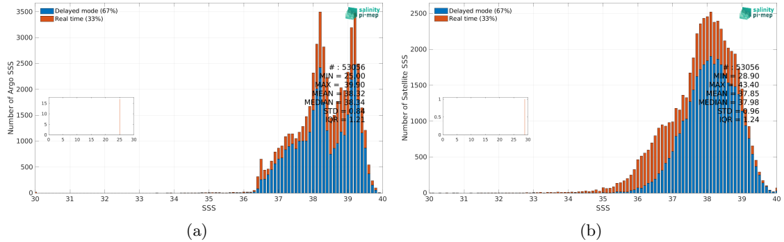
Figure 3: Histograms of SSS from Argo (a) and SMAP SSS L2-AVERAGED v6 (RSS) (b) considering all match-up pairs per bins of 0.1 over the Mediterranean Sea Pi-MEP region and for the full satellite product period.
