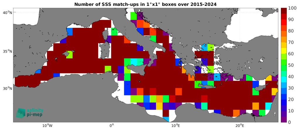
Figure 5: Number of SSS match-ups between Argo SSS and the SMAP SSS L2-AVERAGED v6 (RSS) SSS product for the Mediterranean Sea Pi-MEP region over 1^\circ \times 1^\circ boxes and for the full satellite product period.
