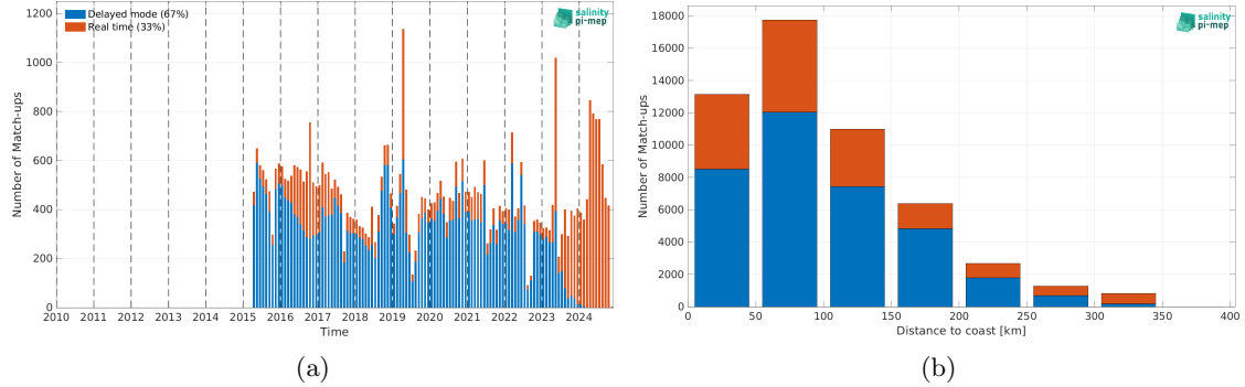
Figure 2: Number of match-ups between Argo and SMAP SSS L2-AVERAGED v6 (RSS) SSS as a function of time (a) and as function of the distance to coast (b) over the Mediterranean Sea Pi-MEP region and for the full satellite product period.
