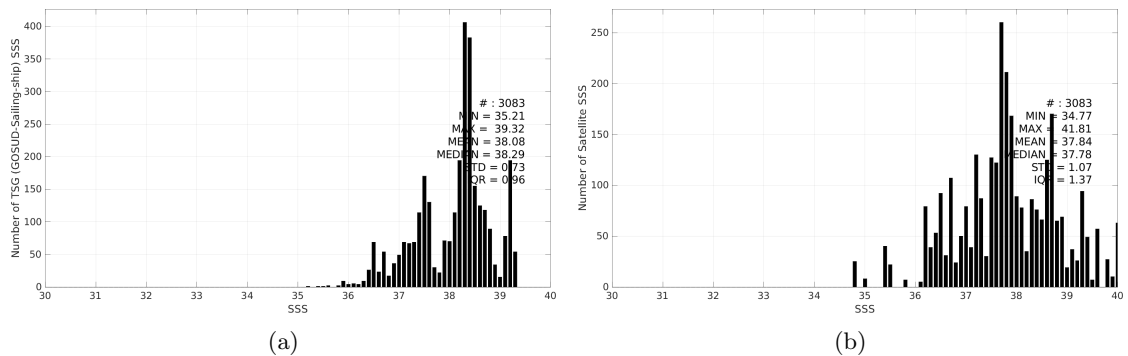
Figure 3: Histograms of SSS from TSG (GOSUD-Sailing-ship) (a) and SMAP SSS L2 v6 (RSS) (b) considering all match-up pairs per bins of 0.1 over the Mediterranean Sea Pi-MEP region and for the full satellite product period.
