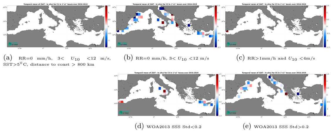
Figure 14: Temporal mean gridded over spatial boxes of size 1^\circ \times 1^\circ of \Delta SSS (SMAP SSS L2 v6 (RSS) - TSG (GOSUD-Sailing-ship)) for 5 different subdatasets corresponding to:RR=0 mm/h, 3 < U_{10} < 12 m/s, SST >5^\circ\text{C} , distance to coast > 800 km (a), RR=0 mm/h, 3 < U_{10} < 12 m/s (b), RR >1 mm/h and U_{10} < 4 m/s (c), WOA2013 SSS Std <0.2 (d), WOA2013 SSS Std >0.2 (e).
