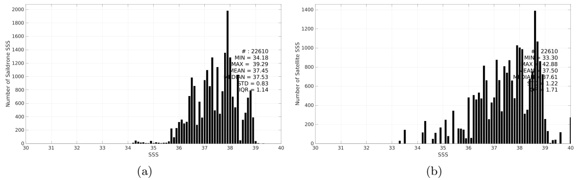
Figure 3: Histograms of SSS from Saildrone (a) and SMAP SSS L2 v6 (RSS) (b) considering all match-up pairs per bins of 0.1 over the Mediterranean Sea Pi-MEP region and for the full satellite product period.
