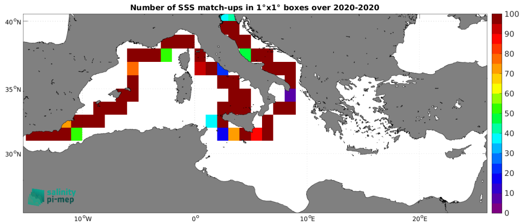
Figure 5: Number of SSS match-ups between Saildrone SSS and the SMAP SSS L2 v6 (RSS) SSS product for the Mediterranean Sea Pi-MEP region over 1^\circ \times 1^\circ boxes and for the full satellite product period.
