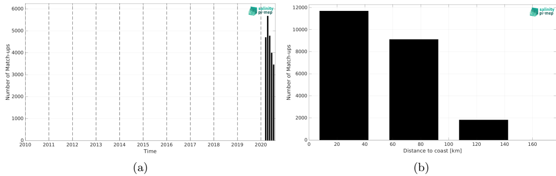
Figure 2: Number of match-ups between Saildrone and SMAP SSS L2 v6 (RSS) SSS as a function of time (a) and as function of the distance to coast (b) over the Mediterranean Sea Pi-MEP region and for the full satellite product period.
