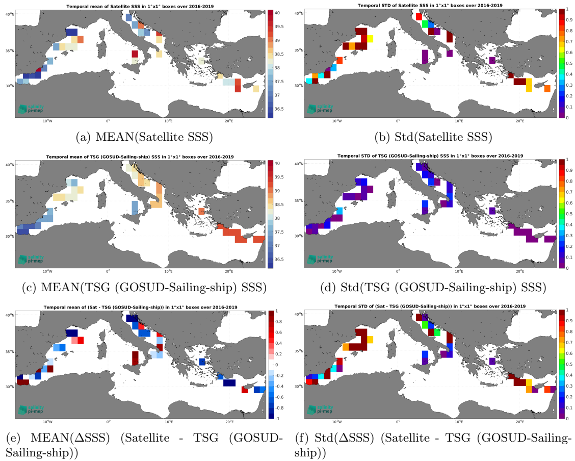
Figure 7: Temporal mean (left) and Std (right) of SSS from SMAP SSS L2 v6 - 40 km (RSS) (top), TSG (GOSUD-Sailing-ship) (middle), and of \Delta SSS (Satellite - TSG (GOSUD-Sailing-ship)). Only match-up pairs are used to generate these maps.
