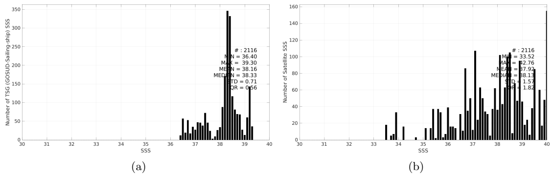
Figure 3: Histograms of SSS from TSG (GOSUD-Sailing-ship) (a) and SMAP SSS L2 v6 - 40 km (RSS) (b) considering all match-up pairs per bins of 0.1 over the Mediterranean Sea Pi-MEP region and for the full satellite product period.
