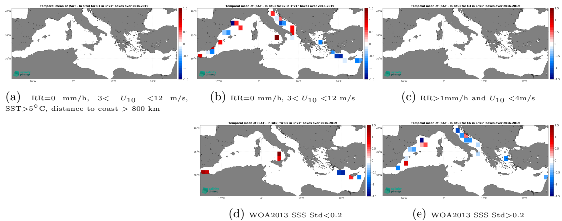
Figure 14: Temporal mean gridded over spatial boxes of size 1^\circ \times 1^\circ of \Delta\text{SSS} (SMAP SSS L2 v6 - 40 km (RSS) - TSG (GOSUD-Sailing-ship)) for 5 different subdatasets corresponding to:RR=0 mm/h, 3 < U_{10} < 12 m/s, SST>5°C, distance to coast > 800 km (a), RR=0 mm/h, 3 < U_{10} < 12 m/s (b), RR>1mm/h and U_{10} < 4 m/s (c), WOA2013 SSS Std<0.2 (d), WOA2013 SSS Std>0.2 (e).
