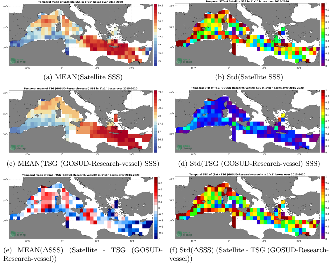
Figure 6: Temporal mean (left) and Std (right) of SSS from SMAP SSS L2 v5 (RSS) (top), TSG (GOSUD-Research-vessel) (middle), and of \Delta SSS (Satellite - TSG (GOSUD-Research-vessel)). Only match-up pairs are used to generate these maps.
