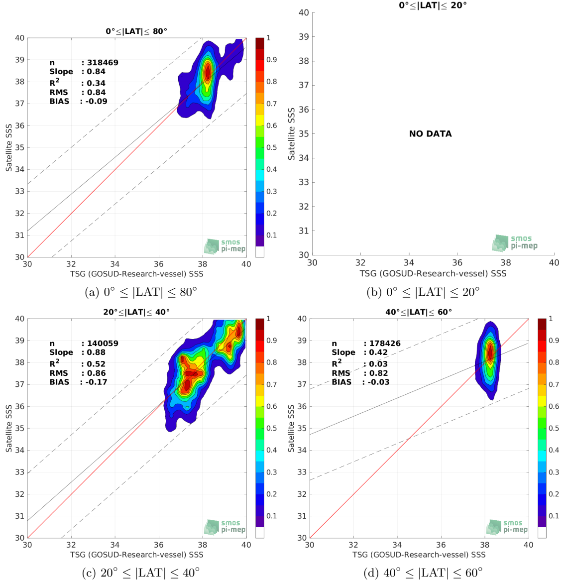
Figure 9: Contour maps of the concentration of SMAP SSS L2 v5 (RSS) SSS (y-axis) versus TSG (GOSUD-Research-vessel) SSS (x-axis) at match-up pairs for different latitude bands. For each plot, the red line shows x=y . The black thin and dashed lines indicate a linear fit through the data cloud and the \pm 95\% confidence levels, respectively. The number match-up pairs n , the slope and R^2 coefficient of the linear fit, the root mean square (RMS) and the mean bias between satellite and in situ data are indicated for each latitude band in each plots.
