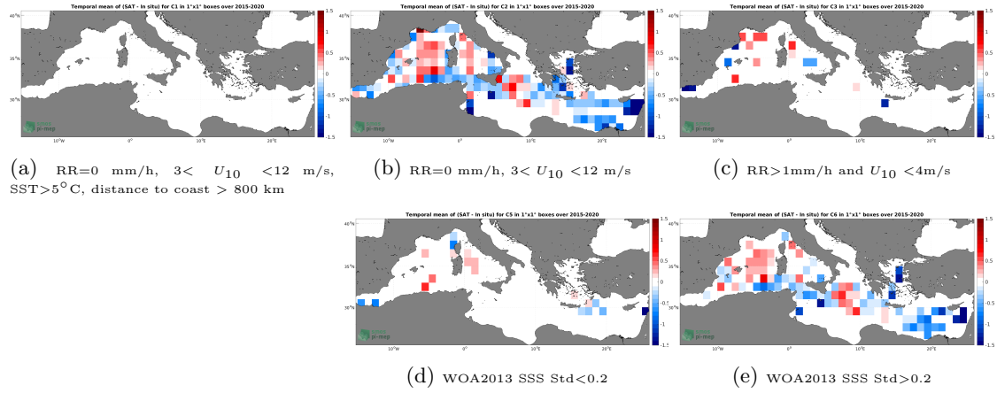
Figure 12: Temporal mean gridded over spatial boxes of size 1^\circ \times 1^\circ of \Delta SSS (SMAP SSS L2 v5 (RSS) - TSG (GOSUD-Research-vessel)) for 5 different subdatasets corresponding to: RR=0 mm/h, 3 < U_{10} < 12 m/s, SST > 5^\circ C , distance to coast > 800 km (a), RR=0 mm/h, 3 < U_{10} < 12 m/s (b), RR > 1 mm/h and U_{10} < 4 m/s (c), WOA2013 SSS Std < 0.2 (d), WOA2013 SSS Std > 0.2 (e).
