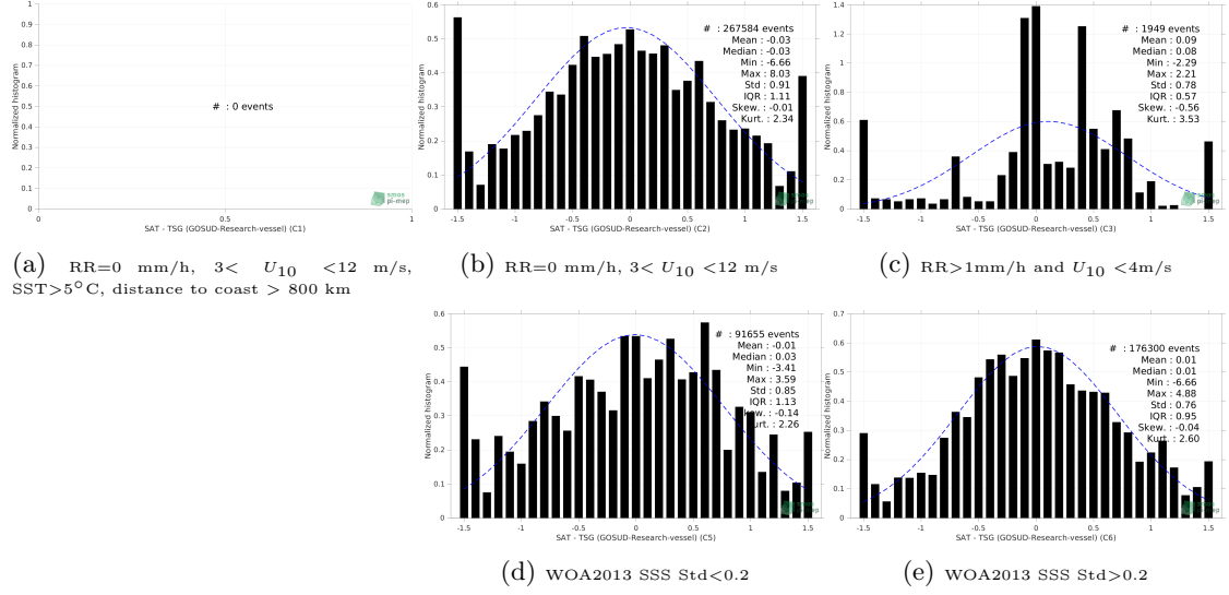
Figure 13: Normalized histogram of \Delta SSS (SMAP SSS L2 v5 (RSS) - TSG (GOSUD-Research-vessel)) for 5 different subdatasets corresponding to: RR=0 mm/h, 3 < U_{10} < 12 m/s, SST>5°C, distance to coast > 800 km (a), RR=0 mm/h, 3 < U_{10} < 12 m/s (b), RR>1mm/h and U_{10} < 4 m/s (c), WOA2013 SSS Std<0.2 (d), WOA2013 SSS Std>0.2 (e).
