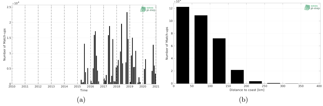
Figure 1: Number of match-ups between TSG (GOSUD-Research-vessel) and SMAP SSS L2 v5 (RSS) SSS as a function of time (a) and as function of the distance to coast (b) over the Mediterranean Sea Pi-MEP region and for the full satellite product period.
