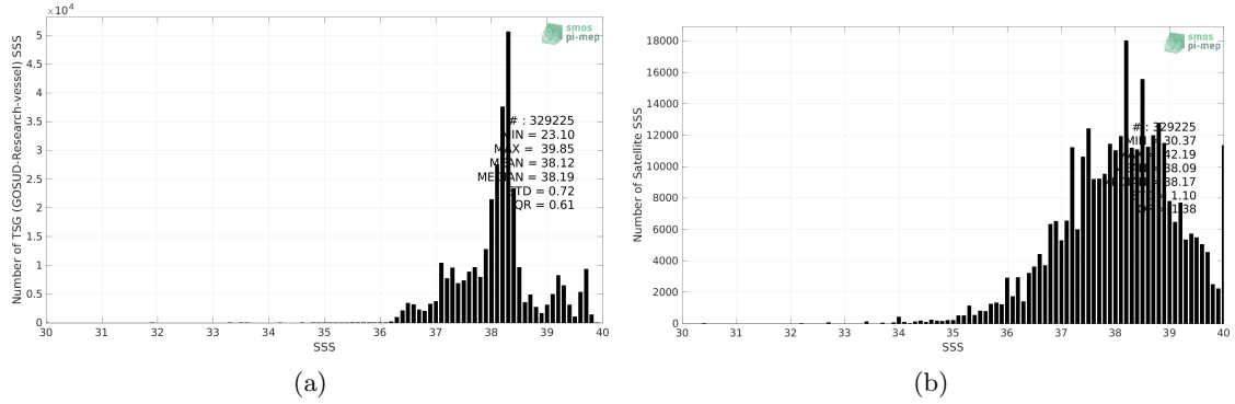
Figure 2: Histograms of SSS from TSG (GOSUD-Research-vessel) (a) and SMAP SSS L2 v5 (RSS) (b) considering all match-up pairs per bins of 0.1 over the Mediterranean Sea Pi-MEP region and for the full satellite product period.
