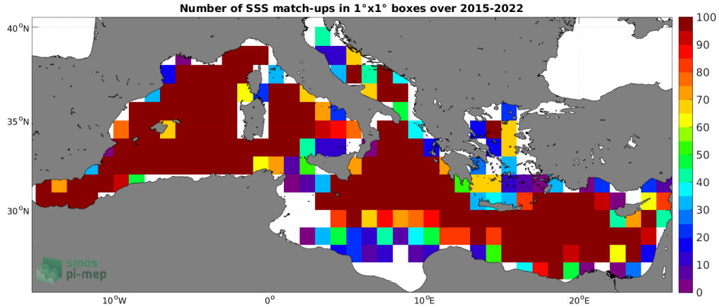
Figure 4: Number of SSS match-ups between Argo SSS and the SMAP SSS L2 v5 (RSS) SSS product for the Mediterranean Sea Pi-MEP region over 1^\circ \times 1^\circ boxes and for the full satellite product period.
