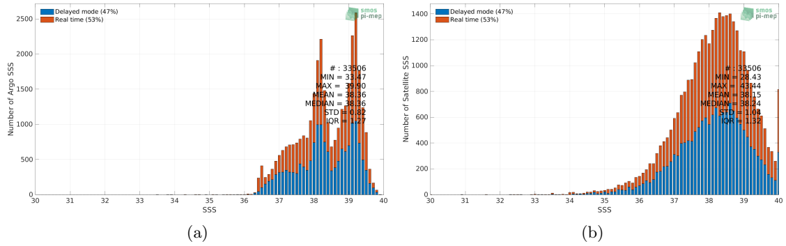
Figure 2: Histograms of SSS from Argo (a) and SMAP SSS L2 v5 (RSS) (b) considering all match-up pairs per bins of 0.1 over the Mediterranean Sea Pi-MEP region and for the full satellite product period.
