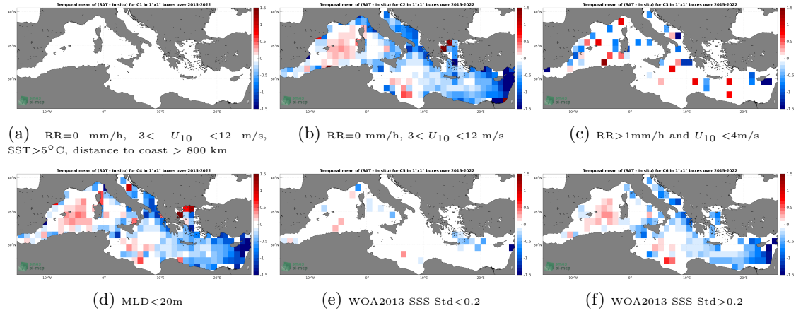
Figure 12: Temporal mean gridded over spatial boxes of size 1^\circ \times 1^\circ of \Delta SSS (SMAP SSS L2 v5 (RSS) - Argo) for 6 different subdatasets corresponding to: RR=0 mm/h, 3 < U_{10} < 12 m/s, SST >5^\circ\text{C} , distance to coast > 800 km (a), RR=0 mm/h, 3 < U_{10} < 12 m/s (b), RR >1 mm/h and U_{10} < 4 m/s (c),MLD <20 m (d),WOA2013 SSS Std <0.2 (e),WOA2013 SSS Std >0.2 (f).
