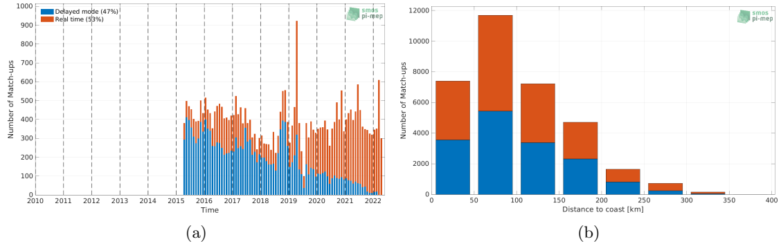
Figure 1: Number of match-ups between Argo and SMAP SSS L2 v5 (RSS) SSS as a function of time (a) and as function of the distance to coast (b) over the Mediterranean Sea Pi-MEP region and for the full satellite product period.
