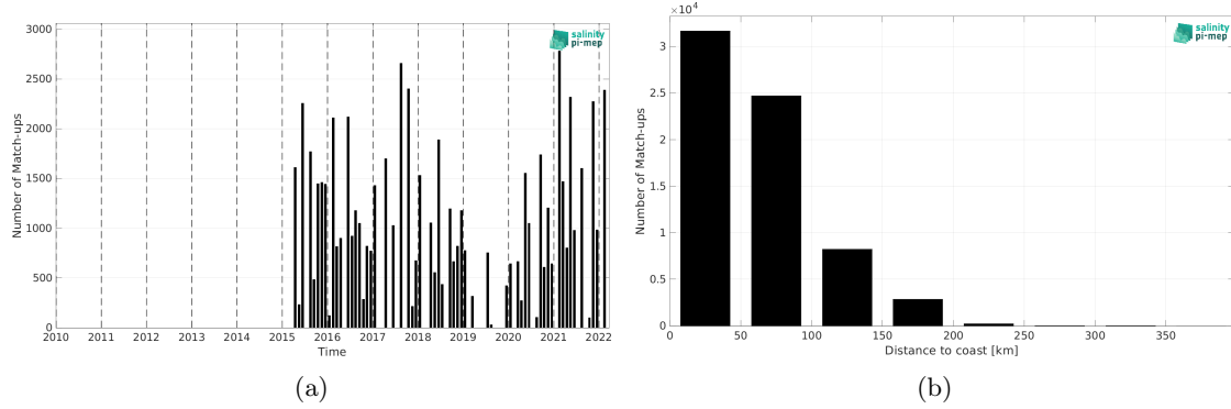
Figure 2: Number of match-ups between TSG (LEGOS-DM) and SMAP SSS L2 v5.3 (RSS) SSS as a function of time (a) and as function of the distance to coast (b) over the Mediterranean Sea Pi-MEP region and for the full satellite product period.
