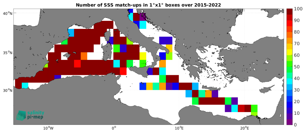
Figure 5: Number of SSS match-ups between TSG (LEGOS-DM) SSS and the SMAP SSS L2 v5.3 (RSS) SSS product for the Mediterranean Sea Pi-MEP region over 1^\circ \times 1^\circ boxes and for the full satellite product period.
