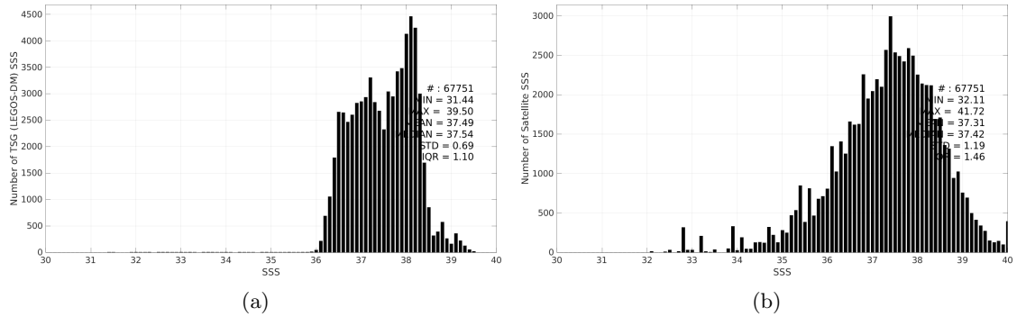
Figure 3: Histograms of SSS from TSG (LEGOS-DM) (a) and SMAP SSS L2 v5.3 (RSS) (b) considering all match-up pairs per bins of 0.1 over the Mediterranean Sea Pi-MEP region and for the full satellite product period.
