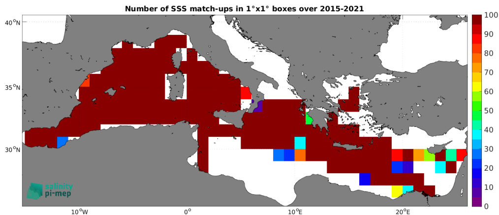
Figure 5: Number of SSS match-ups between TSG (GOSUD-Research-vessel) SSS and the SMAP SSS L2 v5.3 (RSS) SSS product for the Mediterranean Sea Pi-MEP region over 1^\circ \times 1^\circ boxes and for the full satellite product period.
