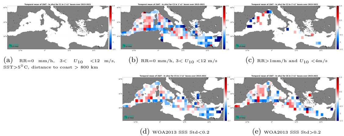
Figure 14: Temporal mean gridded over spatial boxes of size 1^\circ \times 1^\circ of \Delta SSS (SMAP SSS L2 v5.3 (RSS) - TSG (GOSUD-Research-vessel)) for 5 different subdatasets corresponding to:RR=0 mm/h, 3 < U_{10} < 12 m/s, SST >5^\circ C, distance to coast > 800 km (a), RR=0 mm/h, 3 < U_{10} < 12 m/s (b), RR >1 mm/h and U_{10} < 4 m/s (c), WOA2013 SSS Std <0.2 (d), WOA2013 SSS Std >0.2 (e).
