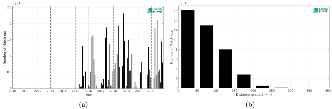
Figure 2: Number of match-ups between TSG (GOSUD-Research-vessel) and SMAP SSS L2 v5.3 (RSS) SSS as a function of time (a) and as function of the distance to coast (b) over the Mediterranean Sea Pi-MEP region and for the full satellite product period.
