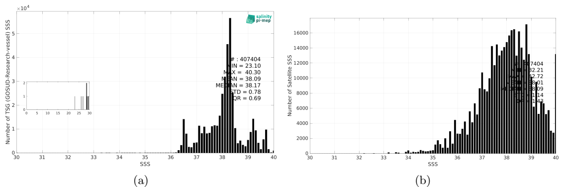
Figure 3: Histograms of SSS from TSG (GOSUD-Research-vessel) (a) and SMAP SSS L2 v5.3 (RSS) (b) considering all match-up pairs per bins of 0.1 over the Mediterranean Sea Pi-MEP region and for the full satellite product period.
