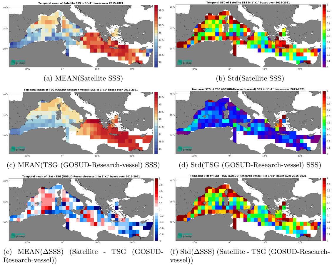
Figure 7: Temporal mean (left) and Std (right) of SSS from SMAP SSS L2 v5.3 (RSS) (top), TSG (GOSUD-Research-vessel) (middle), and of \Delta SSS (Satellite - TSG (GOSUD-Research-vessel)). Only match-up pairs are used to generate these maps.
