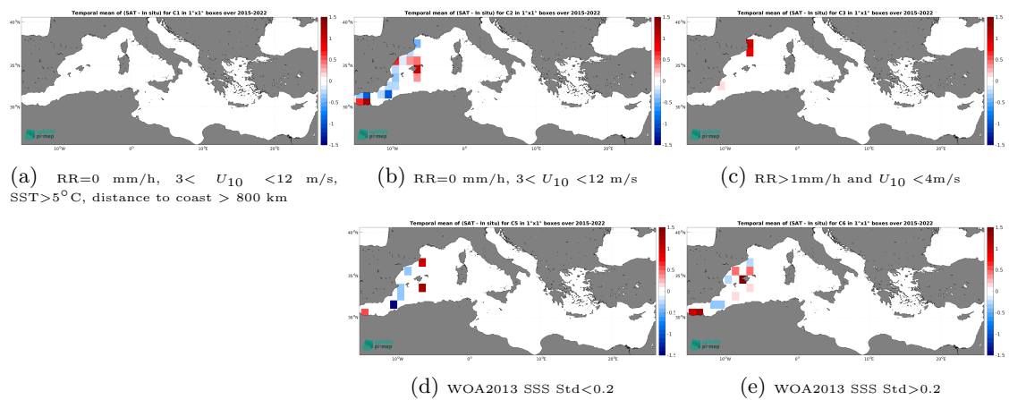
Figure 14: Temporal mean gridded over spatial boxes of size 1^\circ \times 1^\circ of \Delta SSS (SMAP SSS L2 v5.3 (RSS) - TSG (CSIC-UTM)) for 5 different subdatasets corresponding to:RR=0 mm/h, 3 < U_{10} < 12 m/s, SST >5^\circ\text{C} , distance to coast > 800 km (a), RR=0 mm/h, 3 < U_{10} < 12 m/s (b), RR >1 mm/h and U_{10} < 4 m/s (c), WOA2013 SSS Std <0.2 (d), WOA2013 SSS Std >0.2 (e).
