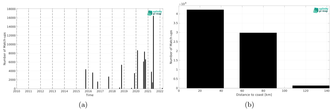
Figure 2: Number of match-ups between TSG (CSIC-UTM) and SMAP SSS L2 v5.3 (RSS) SSS as a function of time (a) and as function of the distance to coast (b) over the Mediterranean Sea Pi-MEP region and for the full satellite product period.
