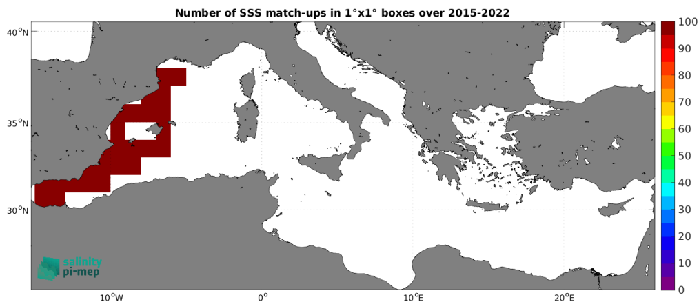
Figure 5: Number of SSS match-ups between TSG (CSIC-UTM) SSS and the SMAP SSS L2 v5.3 (RSS) SSS product for the Mediterranean Sea Pi-MEP region over 1^\circ \times 1^\circ boxes and for the full satellite product period.
