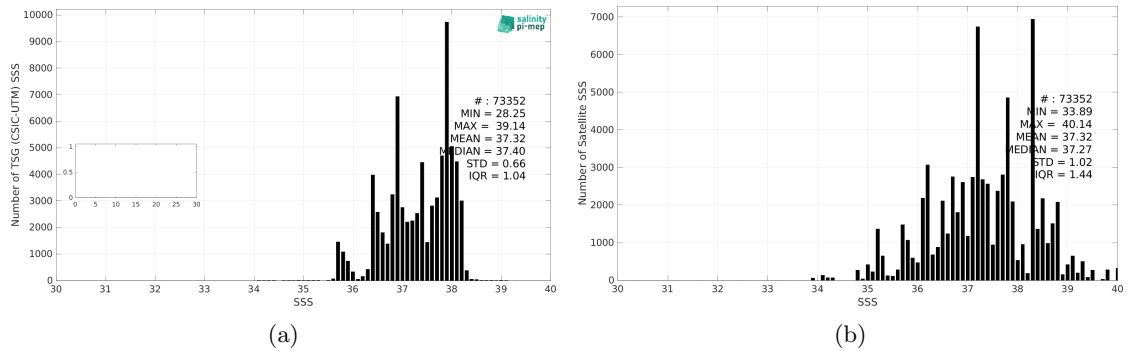
Figure 3: Histograms of SSS from TSG (CSIC-UTM) (a) and SMAP SSS L2 v5.3 (RSS) (b) considering all match-up pairs per bins of 0.1 over the Mediterranean Sea Pi-MEP region and for the full satellite product period.
