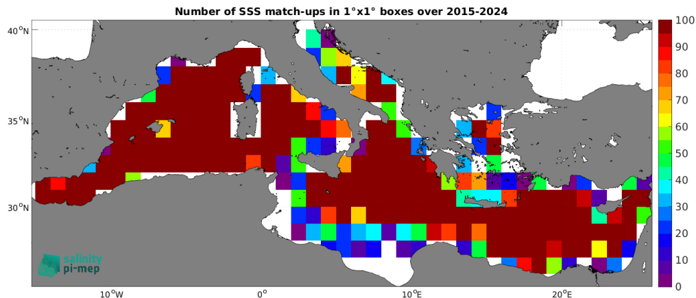
Figure 5: Number of SSS match-ups between Argo SSS and the SMAP SSS L2 v5.3 (RSS) SSS product for the Mediterranean Sea Pi-MEP region over 1^\circ \times 1^\circ boxes and for the full satellite product period.
