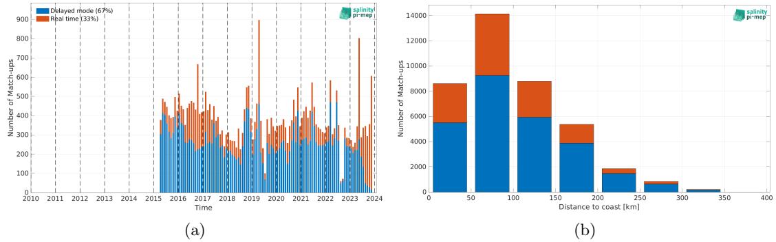
Figure 2: Number of match-ups between Argo and SMAP SSS L2 v5.3 (RSS) SSS as a function of time (a) and as function of the distance to coast (b) over the Mediterranean Sea Pi-MEP region and for the full satellite product period.
