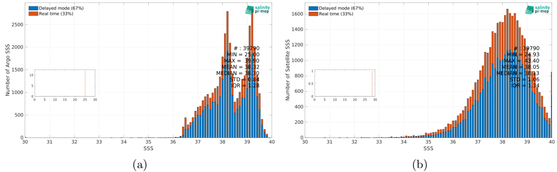
Figure 3: Histograms of SSS from Argo (a) and SMAP SSS L2 v5.3 (RSS) (b) considering all match-up pairs per bins of 0.1 over the Mediterranean Sea Pi-MEP region and for the full satellite product period.
