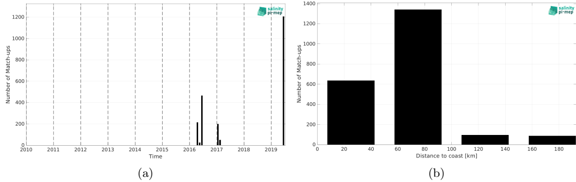
Figure 1: Number of match-ups between TSG (GOSUD-Sailing-ship) and SMAP SSS L2 v5 - 40 km (RSS) SSS as a function of time (a) and as function of the distance to coast (b) over the Mediterranean Sea Pi-MEP region and for the full satellite product period.
