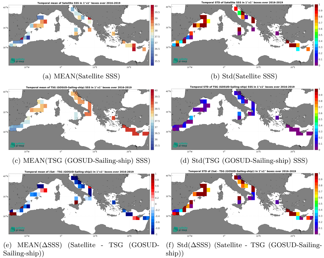
Figure 6: Temporal mean (left) and Std (right) of SSS from SMAP SSS L2 v5 - 40 km (RSS) (top), TSG (GOSUD-Sailing-ship) (middle), and of \Delta SSS (Satellite - TSG (GOSUD-Sailing-ship)). Only match-up pairs are used to generate these maps.
