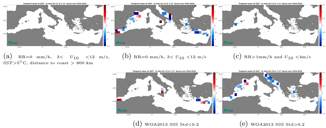
Figure 12: Temporal mean gridded over spatial boxes of size 1^\circ \times 1^\circ of \Delta\text{SSS} (SMAP SSS L2 v5 - 40 km (RSS) - TSG (GOSUD-Sailing-ship)) for 5 different subdatasets corresponding to:RR=0 mm/h, 3 < U_{10} < 12 m/s, SST>5°C, distance to coast > 800 km (a), RR=0 mm/h, 3 < U_{10} < 12 m/s (b), RR>1mm/h and U_{10} < 4 m/s (c), WOA2013 SSS Std<0.2 (d), WOA2013 SSS Std>0.2 (e).
