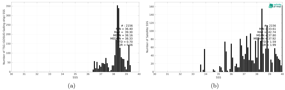
Figure 2: Histograms of SSS from TSG (GOSUD-Sailing-ship) (a) and SMAP SSS L2 v5 - 40 km (RSS) (b) considering all match-up pairs per bins of 0.1 over the Mediterranean Sea Pi-MEP region and for the full satellite product period.
