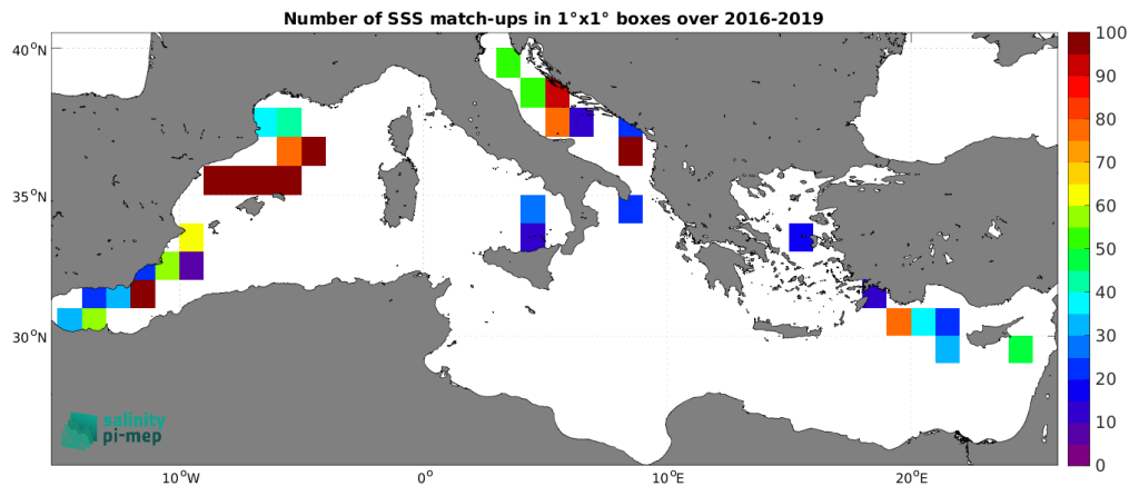
Figure 4: Number of SSS match-ups between TSG (GOSUD-Sailing-ship) SSS and the SMAP SSS L2 v5 - 40 km (RSS) SSS product for the Mediterranean Sea Pi-MEP region over 1^\circ \times 1^\circ boxes and for the full satellite product period.
