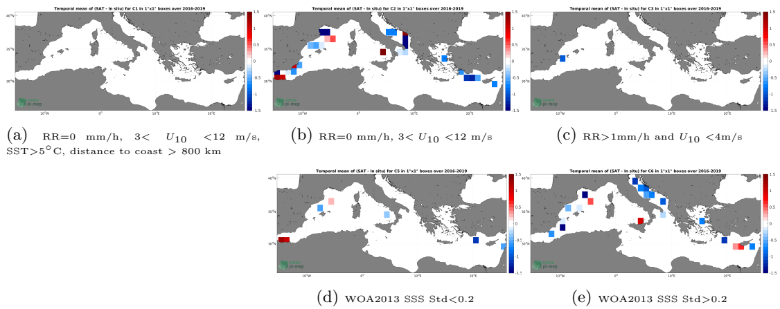
Figure 12: Temporal mean gridded over spatial boxes of size 1^\circ \times 1^\circ of \Delta SSS (SMAP SSS L2 v5 - 40 km (RSS) - TSG (GOSUD-Sailing-ship)) for 5 different subdatasets corresponding to:RR=0 mm/h, 3 < U_{10} < 12 m/s, SST>5°C, distance to coast > 800 km (a), RR=0 mm/h, 3 < U_{10} < 12 m/s (b), RR>1mm/h and U_{10} < 4 m/s (c), WOA2013 SSS Std<0.2 (d), WOA2013 SSS Std>0.2 (e).
