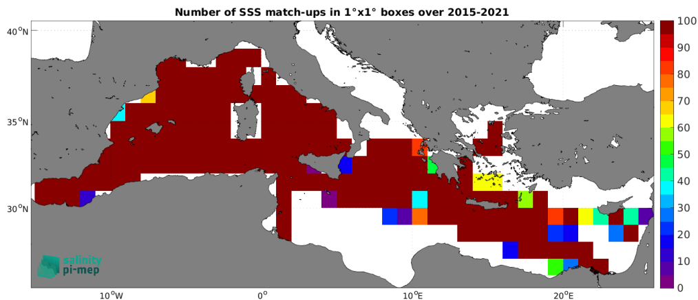
Figure 4: Number of SSS match-ups between TSG (GOSUD-Research-vessel) SSS and the SMAP SSS L2 v5 - 40 km (RSS) SSS product for the Mediterranean Sea Pi-MEP region over 1^\circ \times 1^\circ boxes and for the full satellite product period.
