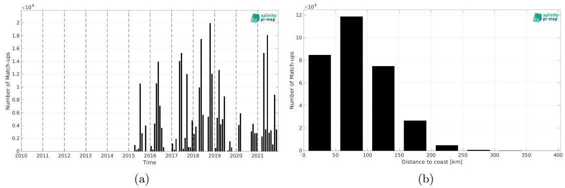
Figure 1: Number of match-ups between TSG (GOSUD-Research-vessel) and SMAP SSS L2 v5 - 40 km (RSS) SSS as a function of time (a) and as function of the distance to coast (b) over the Mediterranean Sea Pi-MEP region and for the full satellite product period.
