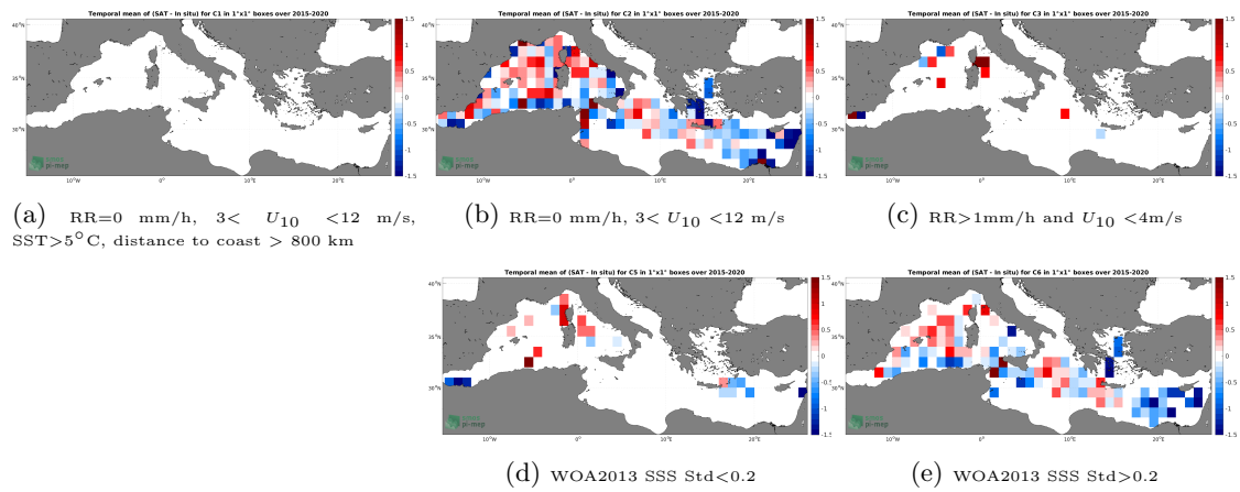
Figure 12: Temporal mean gridded over spatial boxes of size 1^\circ \times 1^\circ of \Delta SSS (SMAP SSS L2 v5 - 40 km (RSS) - TSG (GOSUD-Research-vessel)) for 5 different subdatasets corresponding to:RR=0 mm/h, 3 < U_{10} < 12 m/s, SST>5°C, distance to coast > 800 km (a), RR=0 mm/h, 3 < U_{10} < 12 m/s (b), RR>1mm/h and U_{10} < 4 m/s (c), WOA2013 SSS Std<0.2 (d), WOA2013 SSS Std>0.2 (e).
