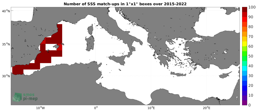
Figure 4: Number of SSS match-ups between TSG (CSIC-UTM) SSS and the SMAP SSS L2 v5 - 40 km (RSS) SSS product for the Mediterranean Sea Pi-MEP region over 1^\circ \times 1^\circ boxes and for the full satellite product period.
