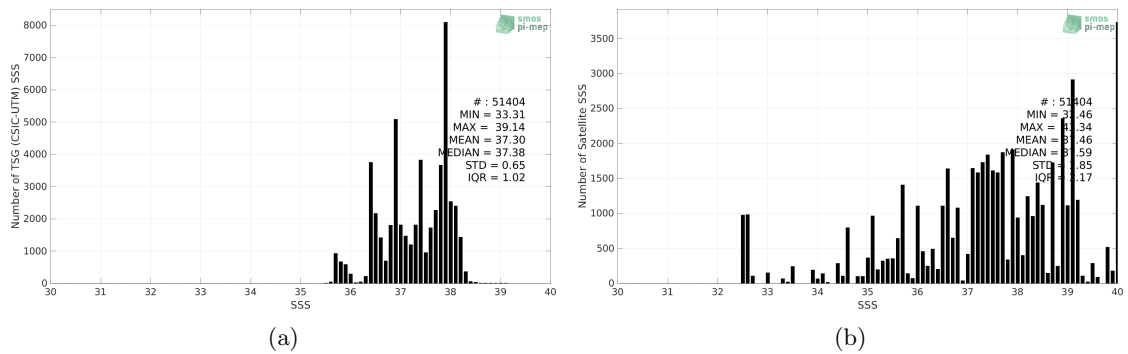
Figure 2: Histograms of SSS from TSG (CSIC-UTM) (a) and SMAP SSS L2 v5 - 40 km (RSS) (b) considering all match-up pairs per bins of 0.1 over the Mediterranean Sea Pi-MEP region and for the full satellite product period.
