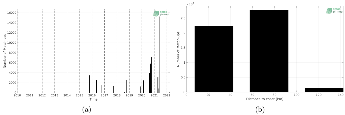
Figure 1: Number of match-ups between TSG (CSIC-UTM) and SMAP SSS L2 v5 - 40 km (RSS) SSS as a function of time (a) and as function of the distance to coast (b) over the Mediterranean Sea Pi-MEP region and for the full satellite product period.
