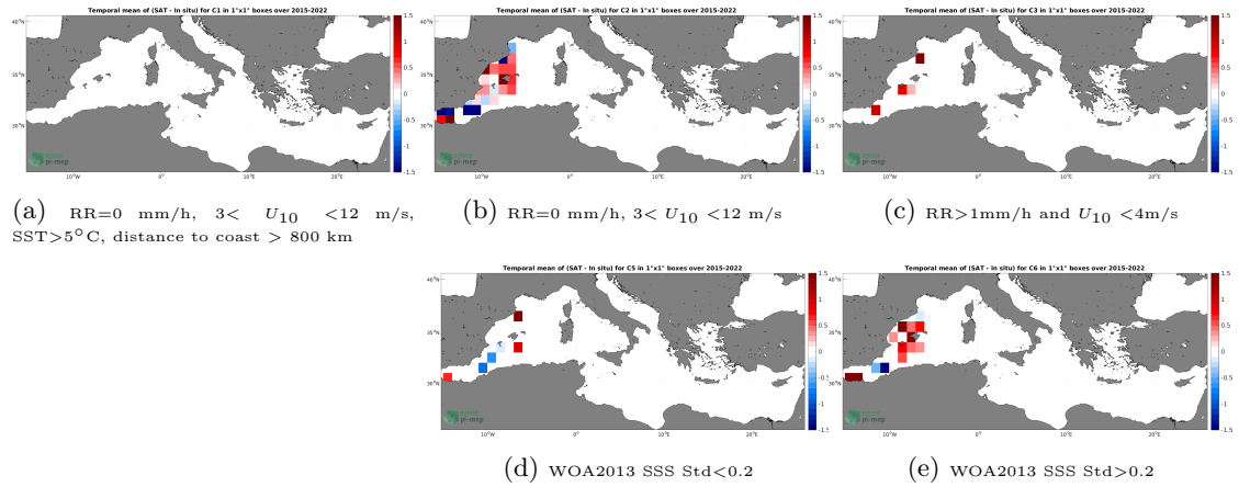
Figure 12: Temporal mean gridded over spatial boxes of size 1^\circ \times 1^\circ of \Delta SSS (SMAP SSS L2 v5 - 40 km (RSS) - TSG (CSIC-UTM)) for 5 different subdatasets corresponding to:RR=0 mm/h, 3 < U_{10} < 12 m/s, SST >5^\circ\text{C} , distance to coast > 800 km (a), RR=0 mm/h, 3 < U_{10} < 12 m/s (b), RR >1 mm/h and U_{10} < 4 m/s (c), WOA2013 SSS Std <0.2 (d), WOA2013 SSS Std >0.2 (e).
