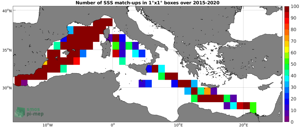
Figure 4: Number of SSS match-ups between TSG (LEGOS-DM) SSS and the SMAP SSS L2 v4 (RSS) SSS product for the Mediterranean Sea Pi-MEP region over 1^\circ \times 1^\circ boxes and for the full satellite product period.
