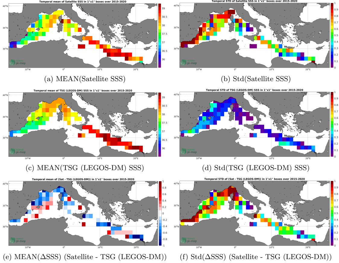
Figure 6: Temporal mean (left) and Std (right) of SSS from SMAP SSS L2 v4 (RSS) (top), TSG (LEGOS-DM) (middle), and of \Delta\text{SSS} (Satellite - TSG (LEGOS-DM)). Only match-up pairs are used to generate these maps.
