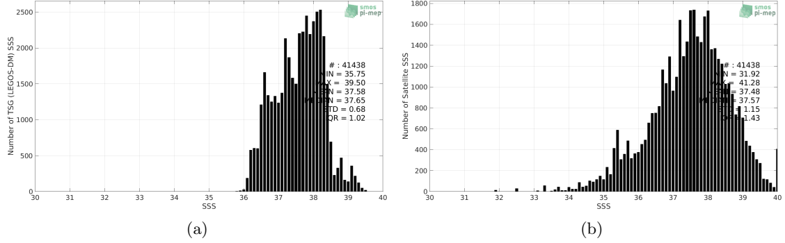
Figure 2: Histograms of SSS from TSG (LEGOS-DM) (a) and SMAP SSS L2 v4 (RSS) (b) considering all match-up pairs per bins of 0.1 over the Mediterranean Sea Pi-MEP region and for the full satellite product period.
