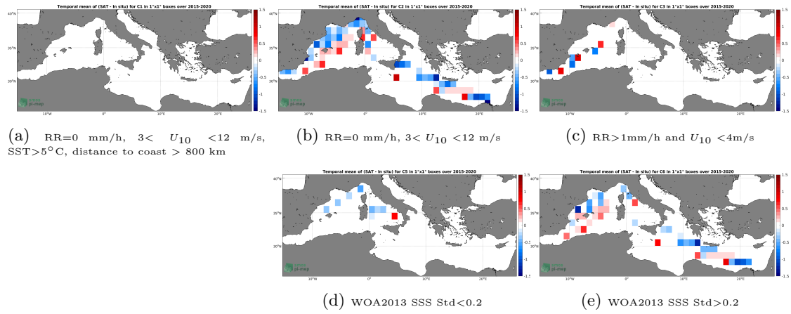
Figure 12: Temporal mean gridded over spatial boxes of size 1^\circ \times 1^\circ of \Delta SSS (SMAP SSS L2 v4 (RSS) - TSG (LEGOS-DM)) for 5 different subdatasets corresponding to: RR=0 mm/h, 3 < U_{10} < 12 m/s, SST > 5^\circ\text{C} , distance to coast > 800 km (a), RR=0 mm/h, 3 < U_{10} < 12 m/s (b), RR > 1 mm/h and U_{10} < 4 m/s (c), WOA2013 SSS Std < 0.2 (d), WOA2013 SSS Std > 0.2 (e).
