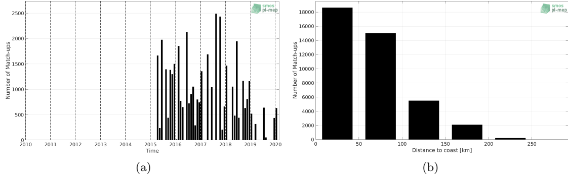
Figure 1: Number of match-ups between TSG (LEGOS-DM) and SMAP SSS L2 v4 (RSS) SSS as a function of time (a) and as function of the distance to coast (b) over the Mediterranean Sea Pi-MEP region and for the full satellite product period.
