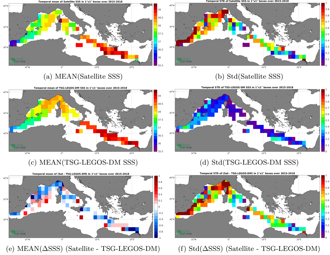
Figure 6: Temporal mean (left) and Std (right) of SSS from SMAP-L2-RSS-V4 (top), TSG-LEGOS-DM (middle), and of \Delta\text{SSS} (Satellite - TSG-LEGOS-DM). Only match-up pairs are used to generate these maps.
