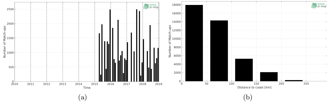
Figure 1: Number of match-ups between TSG-LEGOS-DM and SMAP-L2-RSS-V4 SSS as a function of time (a) and as function of the distance to coast (b) over the Mediterranean Sea Pi-MEP region and for the full satellite product period.
