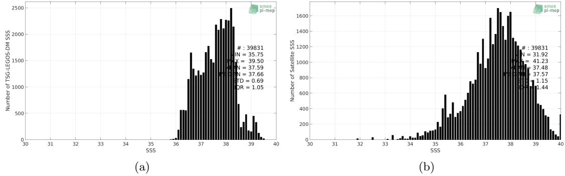
Figure 2: Histograms of SSS from TSG-LEGOS-DM (a) and SMAP-L2-RSS-V4 (b) considering all match-up pairs per bins of 0.1 over the Mediterranean Sea Pi-MEP region and for the full satellite product period.
