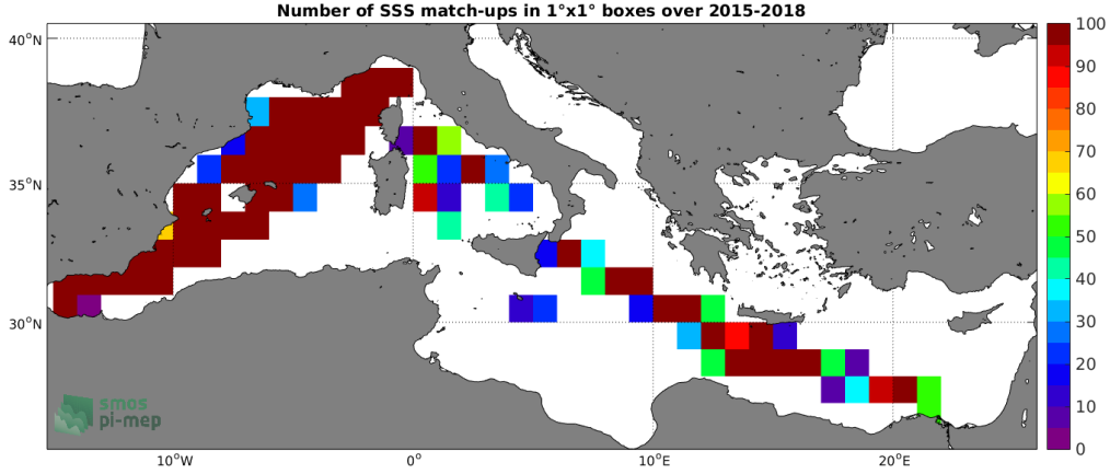
Figure 4: Number of SSS match-ups between TSG-LEGOS-DM SSS and the SMAP-L2-RSS-V4 SSS product for the Mediterranean Sea Pi-MEP region over 1^\circ \times 1^\circ boxes and for the full satellite product period.
