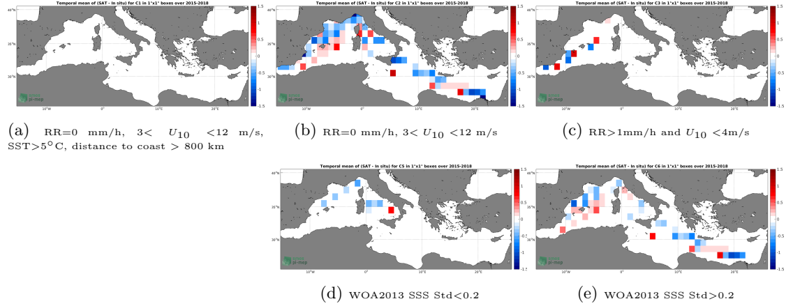
Figure 12: Temporal mean gridded over spatial boxes of size 1^\circ \times 1^\circ of \Delta SSS (SMAP-L2-RSS-V4 - TSG-LEGOS-DM) for 5 different subdatasets corresponding to: RR=0 mm/h, 3 < U_{10} < 12 m/s, SST>5°C, distance to coast > 800 km (a), RR=0 mm/h, 3 < U_{10} < 12 m/s (b), RR>1mm/h and U_{10} < 4 m/s (c), WOA2013 SSS Std<0.2 (d), WOA2013 SSS Std>0.2 (e).
