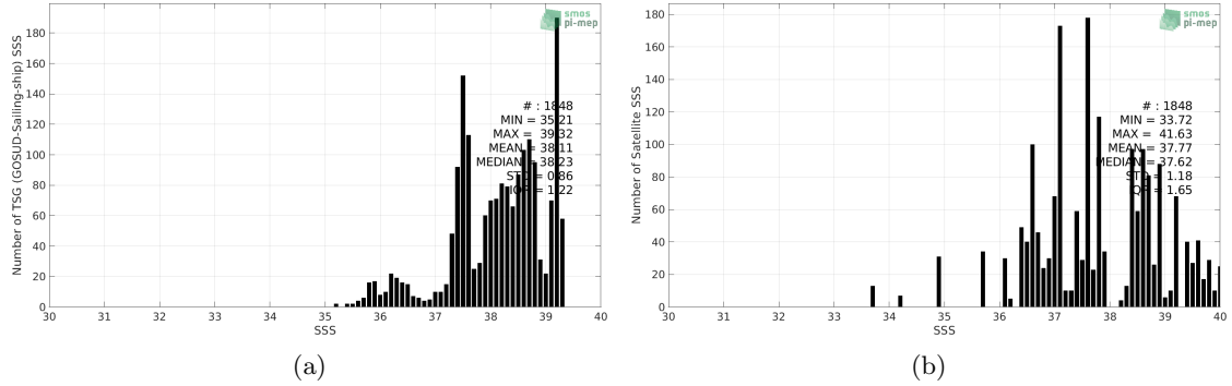
Figure 2: Histograms of SSS from TSG (GOSUD-Sailing-ship) (a) and SMAP SSS L2 v4 (RSS) (b) considering all match-up pairs per bins of 0.1 over the Mediterranean Sea Pi-MEP region and for the full satellite product period.
