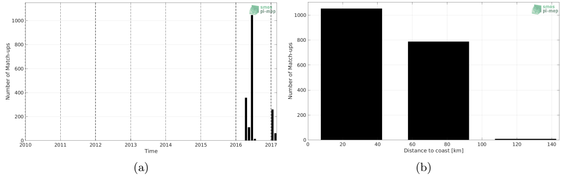
Figure 1: Number of match-ups between TSG (GOSUD-Sailing-ship) and SMAP SSS L2 v4 (RSS) SSS as a function of time (a) and as function of the distance to coast (b) over the Mediterranean Sea Pi-MEP region and for the full satellite product period.
