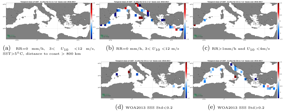
Figure 12: Temporal mean gridded over spatial boxes of size 1^\circ \times 1^\circ of \Delta SSS (SMAP SSS L2 v4 (RSS) - TSG (GOSUD-Sailing-ship)) for 5 different subdatasets corresponding to: RR=0 mm/h, 3 < U_{10} < 12 m/s, SST > 5^\circ C , distance to coast > 800 km (a), RR=0 mm/h, 3 < U_{10} < 12 m/s (b), RR > 1 mm/h and U_{10} < 4 m/s (c), WOA2013 SSS Std < 0.2 (d), WOA2013 SSS Std > 0.2 (e).
