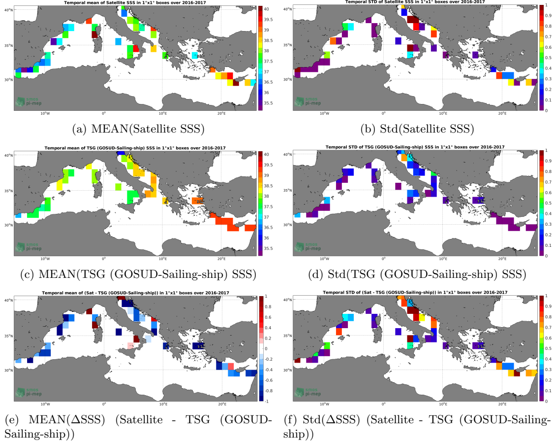
Figure 6: Temporal mean (left) and Std (right) of SSS from SMAP SSS L2 v4 (RSS) (top), TSG (GOSUD-Sailing-ship) (middle), and of \Delta\text{SSS} (Satellite - TSG (GOSUD-Sailing-ship)). Only match-up pairs are used to generate these maps.
