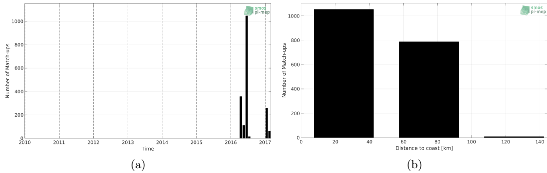
Figure 1: Number of match-ups between TSG-GOSUD-Sailing-ship and SMAP-L2-RSS-V4 SSS as a function of time (a) and as function of the distance to coast (b) over the Mediterranean Sea Pi-MEP region and for the full satellite product period.
