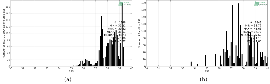
Figure 2: Histograms of SSS from TSG-GOSUD-Sailing-ship (a) and SMAP-L2-RSS-V4 (b) considering all match-up pairs per bins of 0.1 over the Mediterranean Sea Pi-MEP region and for the full satellite product period.
