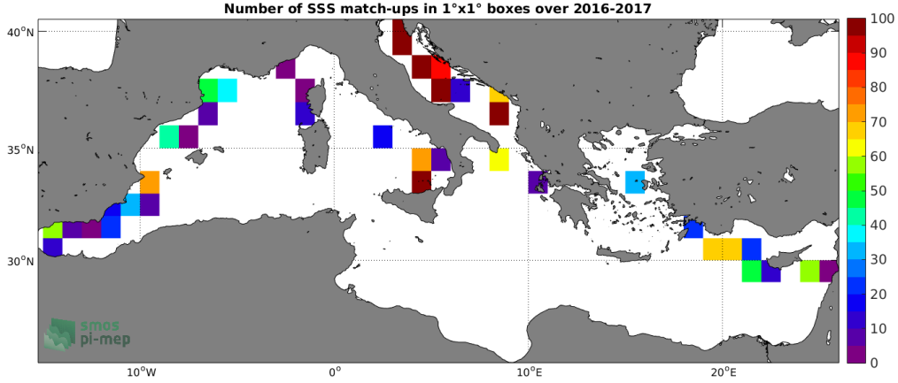
Figure 4: Number of SSS match-ups between TSG-GOSUD-Sailing-ship SSS and the SMAP-L2-RSS-V4 SSS product for the Mediterranean Sea Pi-MEP region over 1^\circ \times 1^\circ boxes and for the full satellite product period.
