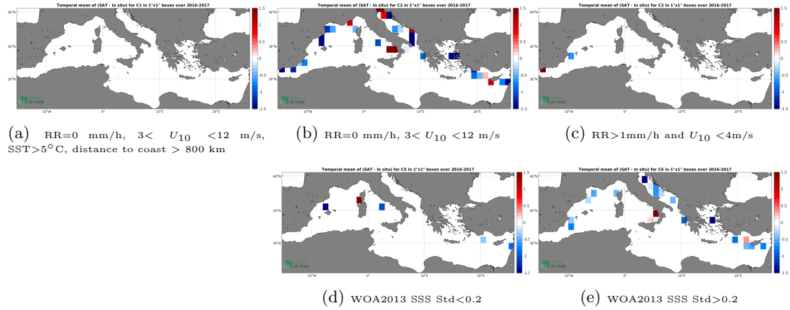
Figure 12: Temporal mean gridded over spatial boxes of size 1^\circ \times 1^\circ of \Delta SSS (SMAP-L2-RSS-V4 - TSG-GOSUD-Sailing-ship) for 5 different subdatasets corresponding to: RR=0 mm/h, 3 < U_{10} < 12 m/s, SST >5^\circ\text{C} , distance to coast > 800 km (a), RR=0 mm/h, 3 < U_{10} < 12 m/s (b), RR >1 mm/h and U_{10} < 4 m/s (c), WOA2013 SSS Std <0.2 (d), WOA2013 SSS Std >0.2 (e).
