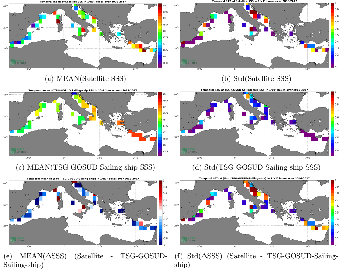
Figure 6: Temporal mean (left) and Std (right) of SSS from SMAP-L2-RSS-V4 (top), TSG-GOSUD-Sailing-ship (middle), and of \Delta\text{SSS} (Satellite - TSG-GOSUD-Sailing-ship). Only match-up pairs are used to generate these maps.
