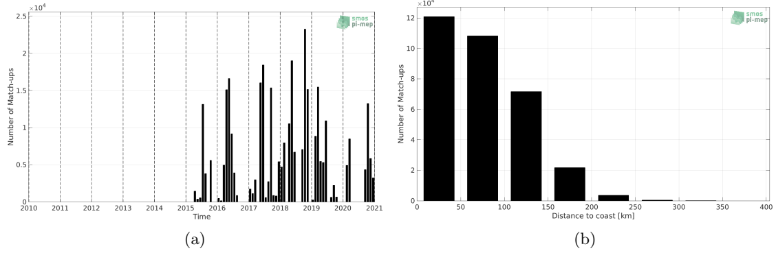
Figure 1: Number of match-ups between TSG (GOSUD-Research-vessel) and SMAP SSS L2 v4 (RSS) SSS as a function of time (a) and as function of the distance to coast (b) over the Mediterranean Sea Pi-MEP region and for the full satellite product period.
