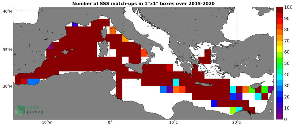
Figure 4: Number of SSS match-ups between TSG (GOSUD-Research-vessel) SSS and the SMAP SSS L2 v4 (RSS) SSS product for the Mediterranean Sea Pi-MEP region over 1^\circ \times 1^\circ boxes and for the full satellite product period.
