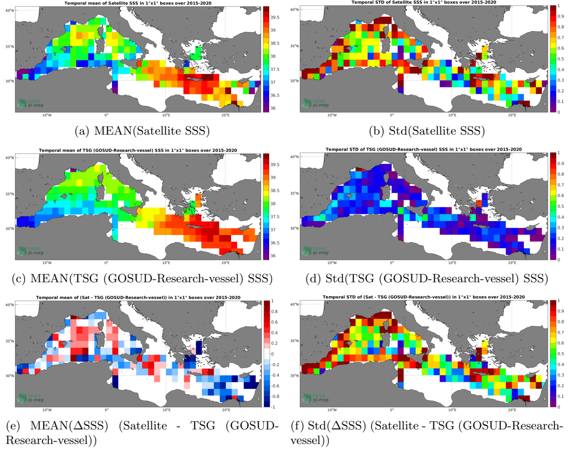
Figure 6: Temporal mean (left) and Std (right) of SSS from SMAP SSS L2 v4 (RSS) (top), TSG (GOSUD-Research-vessel) (middle), and of \Delta SSS (Satellite - TSG (GOSUD-Research-vessel)). Only match-up pairs are used to generate these maps.
