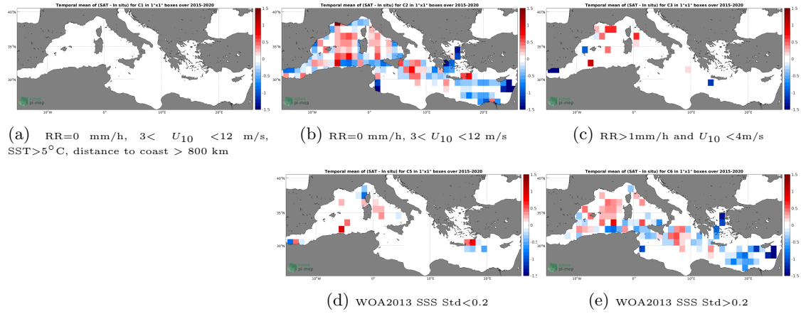
Figure 12: Temporal mean gridded over spatial boxes of size 1^\circ \times 1^\circ of \Delta SSS (SMAP SSS L2 v4 (RSS) - TSG (GOSUD-Research-vessel)) for 5 different subdatasets corresponding to: RR=0 mm/h, 3 < U_{10} < 12 m/s, SST >5^\circ\text{C} , distance to coast > 800 km (a), RR=0 mm/h, 3 < U_{10} < 12 m/s (b), RR >1 mm/h and U_{10} < 4 m/s (c), WOA2013 SSS Std <0.2 (d), WOA2013 SSS Std >0.2 (e).
