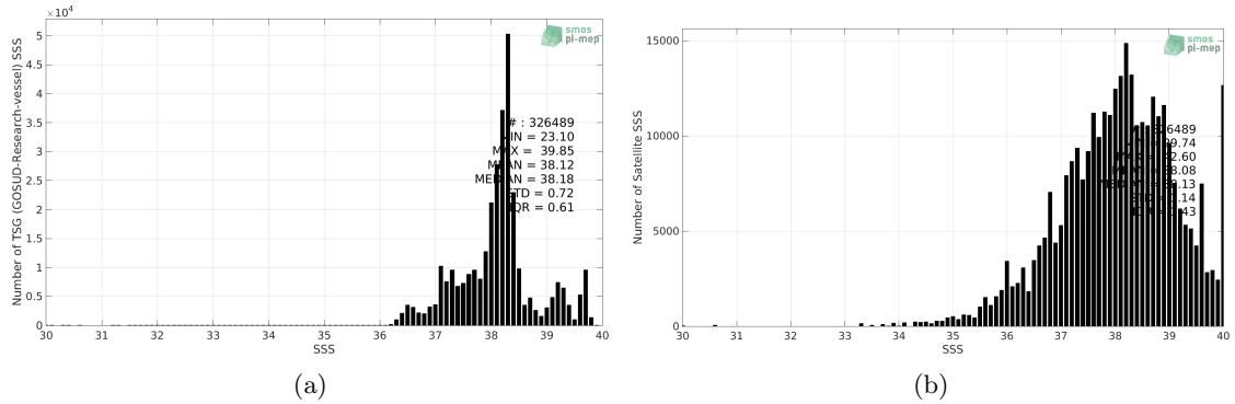
Figure 2: Histograms of SSS from TSG (GOSUD-Research-vessel) (a) and SMAP SSS L2 v4 (RSS) (b) considering all match-up pairs per bins of 0.1 over the Mediterranean Sea Pi-MEP region and for the full satellite product period.
