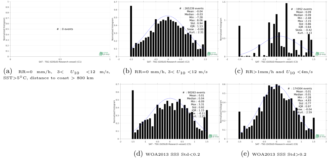
Figure 13: Normalized histogram of \Delta\text{SSS} (SMAP SSS L2 v4 (RSS) - TSG (GOSUD-Research-vessel)) for 5 different subdatasets corresponding to: RR=0 mm/h, 3 < U_{10} < 12 m/s, SST > 5^\circ\text{C} , distance to coast > 800 km (a), RR=0 mm/h, 3 < U_{10} < 12 m/s (b), RR > 1\text{mm/h} and U_{10} < 4\text{m/s} (c), WOA2013 SSS Std <0.2 (d), WOA2013 SSS Std >0.2 (e).
