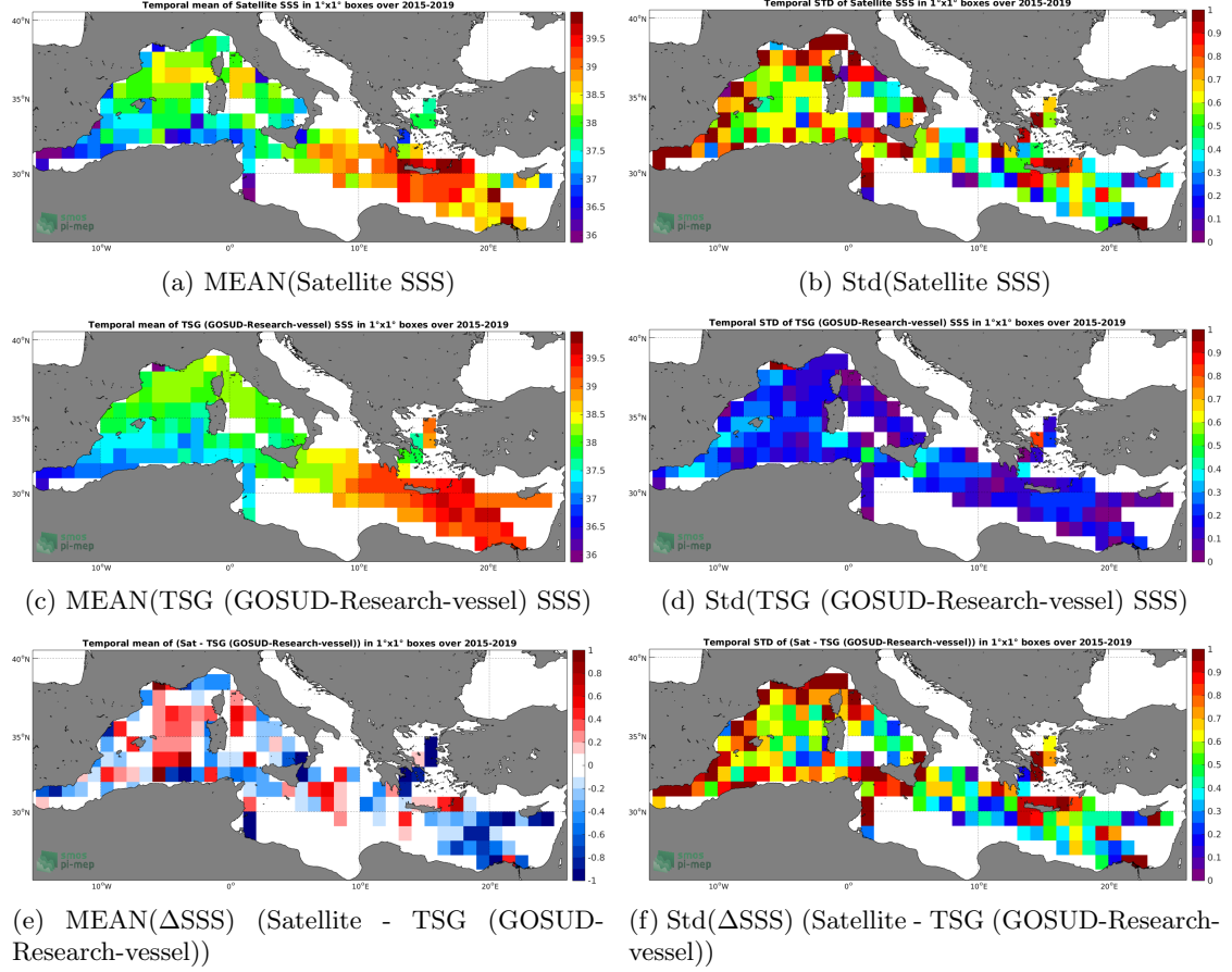
Figure 6: Temporal mean (left) and Std (right) of SSS from SMAP SSS L2 v4 (RSS) (top), TSG (GOSUD-Research-vessel) (middle), and of \Delta\text{SSS} (Satellite - TSG (GOSUD-Research-vessel)). Only match-up pairs are used to generate these maps.
