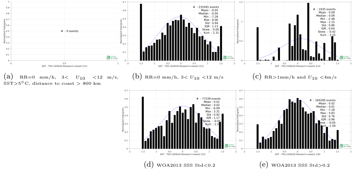
Figure 13: Normalized histogram of \Delta SSS (SMAP SSS L2 v4 (RSS) - TSG (GOSUD-Research-vessel)) for 5 different subdatasets corresponding to: RR=0 mm/h, 3 < U_{10} < 12 m/s, SST > 5^\circ C , distance to coast > 800 km (a), RR=0 mm/h, 3 < U_{10} < 12 m/s (b), RR > 1 mm/h and U_{10} < 4 m/s (c), WOA2013 SSS Std < 0.2 (d), WOA2013 SSS Std > 0.2 (e).
