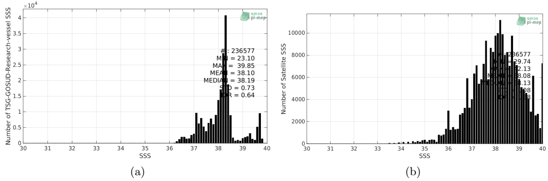
Figure 2: Histograms of SSS from TSG-GOSUD-Research-vessel (a) and SMAP-L2-RSS-V4 (b) considering all match-up pairs per bins of 0.1 over the Mediterranean Sea Pi-MEP region and for the full satellite product period.
