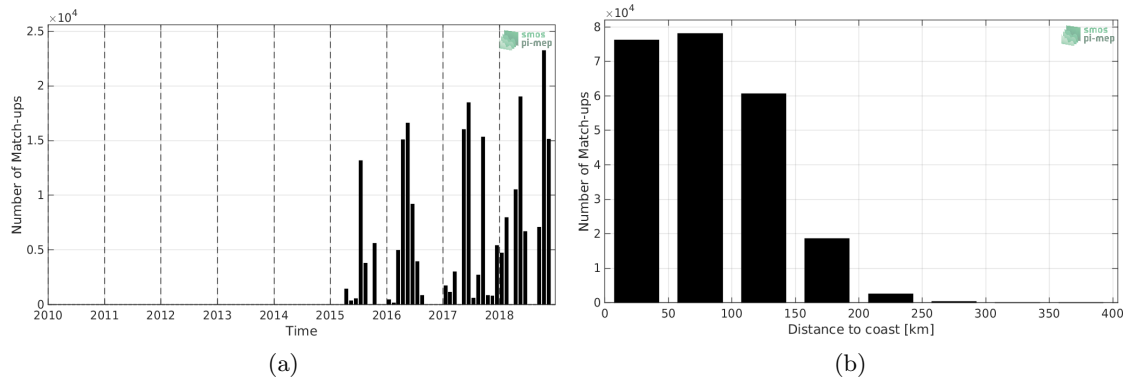
Figure 1: Number of match-ups between TSG-GOSUD-Research-vessel and SMAP-L2-RSS-V4 SSS as a function of time (a) and as function of the distance to coast (b) over the Mediterranean Sea Pi-MEP region and for the full satellite product period.
