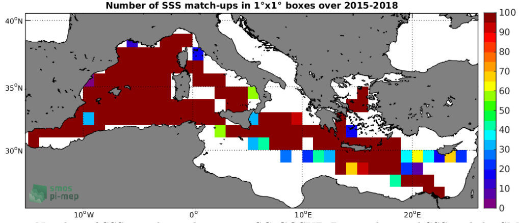
Figure 4: Number of SSS match-ups between TSG-GOSUD-Research-vessel SSS and the SMAP-L2-RSS-V4 SSS product for the Mediterranean Sea Pi-MEP region over 1^\circ \times 1^\circ boxes and for the full satellite product period.
