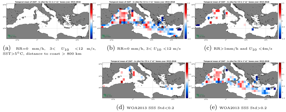
Figure 12: Temporal mean gridded over spatial boxes of size 1^\circ \times 1^\circ of \Delta SSS (SMAP-L2-RSS-V4 - TSG-GOSUD-Research-vessel) for 5 different subdatasets corresponding to:RR=0 mm/h, 3 < U_{10} < 12 m/s, SST >5^\circ\text{C} , distance to coast > 800 km (a), RR=0 mm/h, 3 < U_{10} < 12 m/s (b), RR >1 mm/h and U_{10} < 4 m/s (c), WOA2013 SSS Std <0.2 (d), WOA2013 SSS Std >0.2 (e).
