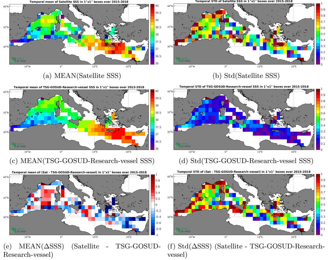
Figure 6: Temporal mean (left) and Std (right) of SSS from SMAP-L2-RSS-V4 (top), TSG-GOSUD-Research-vessel (middle), and of \Delta SSS (Satellite - TSG-GOSUD-Research-vessel). Only match-up pairs are used to generate these maps.
