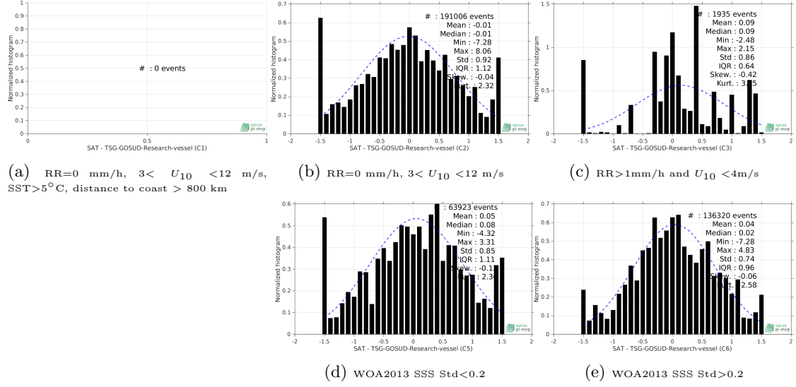
Figure 13: Normalized histogram of \Delta\text{SSS} (SMAP-L2-RSS-V4 - TSG-GOSUD-Research-vessel) for 5 different subdatasets corresponding to: RR=0 mm/h, 3 < U_{10} < 12 m/s, SST > 5^{\circ}\text{C} , distance to coast > 800 km (a), RR=0 mm/h, 3 < U_{10} < 12 m/s (b), RR > 1\text{mm/h} and U_{10} < 4\text{m/s} (c), WOA2013 SSS Std <0.2 (d), WOA2013 SSS Std >0.2 (e).
