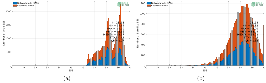
Figure 2: Histograms of SSS from Argo (a) and SMAP SSS L2 v4 (RSS) (b) considering all match-up pairs per bins of 0.1 over the Mediterranean Sea Pi-MEP region and for the full satellite product period.
