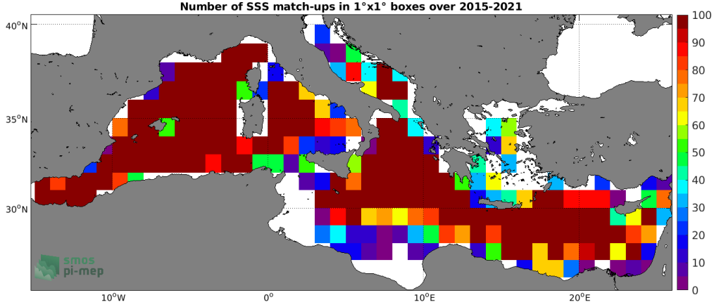
Figure 4: Number of SSS match-ups between Argo SSS and the SMAP SSS L2 v4 (RSS) SSS product for the Mediterranean Sea Pi-MEP region over 1^\circ \times 1^\circ boxes and for the full satellite product period.
