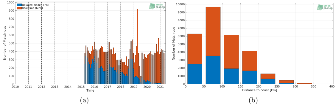
Figure 1: Number of match-ups between Argo and SMAP SSS L2 v4 (RSS) SSS as a function of time (a) and as function of the distance to coast (b) over the Mediterranean Sea Pi-MEP region and for the full satellite product period.
