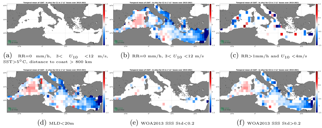
Figure 12: Temporal mean gridded over spatial boxes of size 1^\circ \times 1^\circ of \Delta SSS (SMAP SSS L2 v4 (RSS) - Argo) for 6 different subdatasets corresponding to: RR=0 mm/h, 3 < U_{10} < 12 m/s, SST > 5^\circ C , distance to coast > 800 km (a), RR=0 mm/h, 3 < U_{10} < 12 m/s (b), RR > 1 mm/h and U_{10} < 4 m/s (c), MLD < 20 m (d), WOA2013 SSS Std < 0.2 (e), WOA2013 SSS Std > 0.2 (f).
