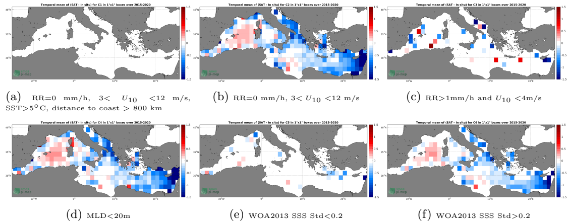
Figure 12: Temporal mean gridded over spatial boxes of size 1^\circ \times 1^\circ of \Delta SSS (SMAP SSS L2 v4 (RSS) - Argo) for 6 different subdatasets corresponding to: RR=0 mm/h, 3 < U_{10} < 12 m/s, SST > 5^\circ C , distance to coast > 800 km (a), RR=0 mm/h, 3 < U_{10} < 12 m/s (b), RR > 1 mm/h and U_{10} < 4 m/s (c), MLD < 20 m (d), WOA2013 SSS Std < 0.2 (e), WOA2013 SSS Std > 0.2 (f).
