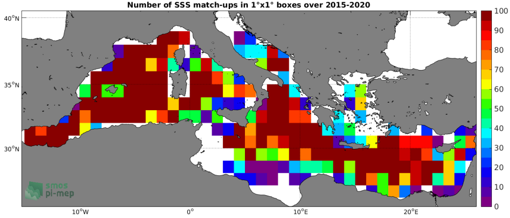
Figure 4: Number of SSS match-ups between Argo SSS and the SMAP-L2-RSS-V4 SSS product for the Mediterranean Sea Pi-MEP region over 1^\circ \times 1^\circ boxes and for the full satellite product period.
