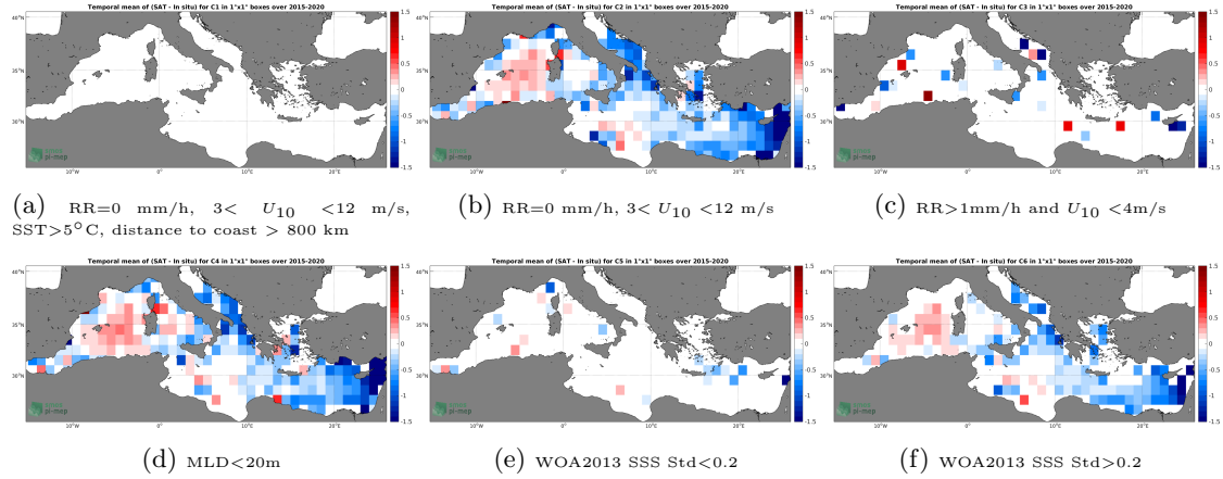
Figure 12: Temporal mean gridded over spatial boxes of size 1^\circ \times 1^\circ of \Delta SSS (SMAP-L2-RSS-V4 - Argo) for 6 different subdatasets corresponding to: RR=0 mm/h, 3 < U_{10} < 12 m/s, SST > 5^\circ C , distance to coast > 800 km (a), RR=0 mm/h, 3 < U_{10} < 12 m/s (b), RR > 1 mm/h and U_{10} < 4 m/s (c), MLD < 20 m (d), WOA2013 SSS Std < 0.2 (e), WOA2013 SSS Std > 0.2 (f).
