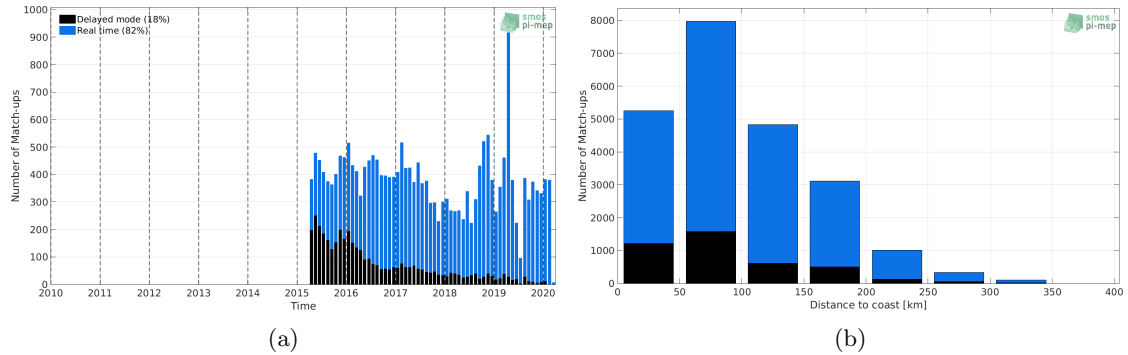
Figure 1: Number of match-ups between Argo and SMAP-L2-RSS-V4 SSS as a function of time (a) and as function of the distance to coast (b) over the Mediterranean Sea Pi-MEP region and for the full satellite product period.
