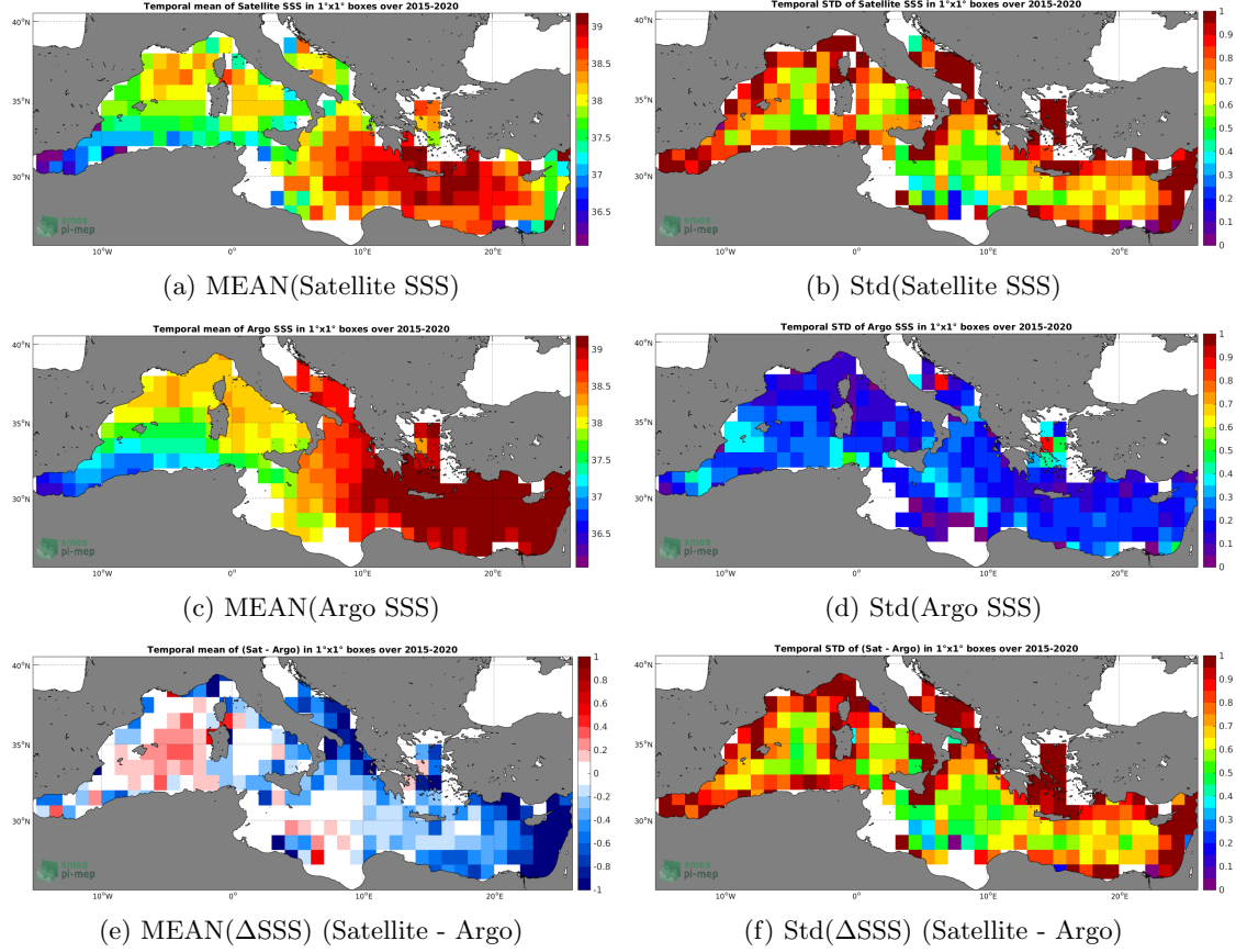
Figure 6: Temporal mean (left) and Std (right) of SSS from SMAP-L2-RSS-V4 (top), Argo (middle), and of \Delta\text{SSS} (Satellite - Argo). Only match-up pairs are used to generate these maps.
