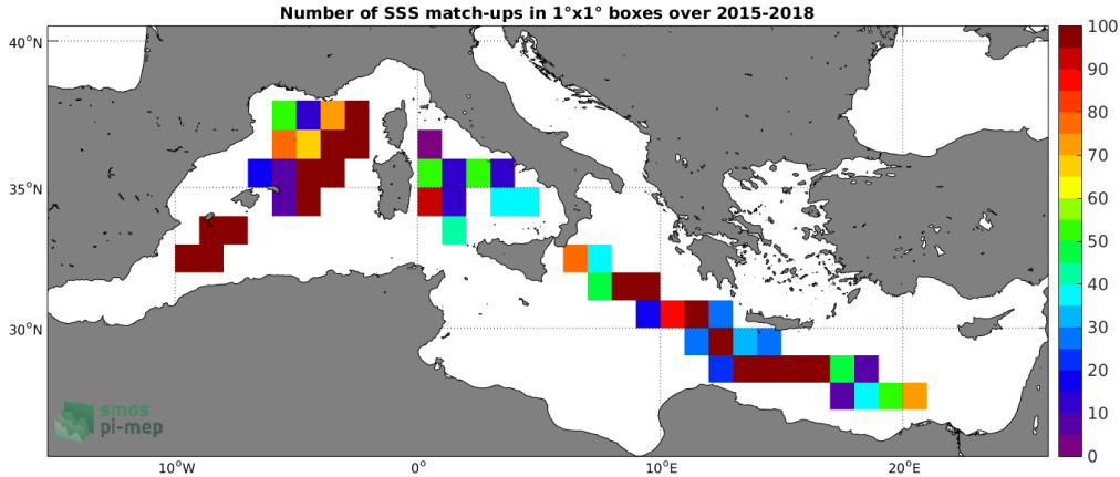
Figure 4: Number of SSS match-ups between TSG-LEGOS-DM SSS and the SMAP-L2-RSS-V3-70KM SSS product for the Mediterranean Sea Pi-MEP region over 1^\circ \times 1^\circ boxes and for the full satellite product period.
