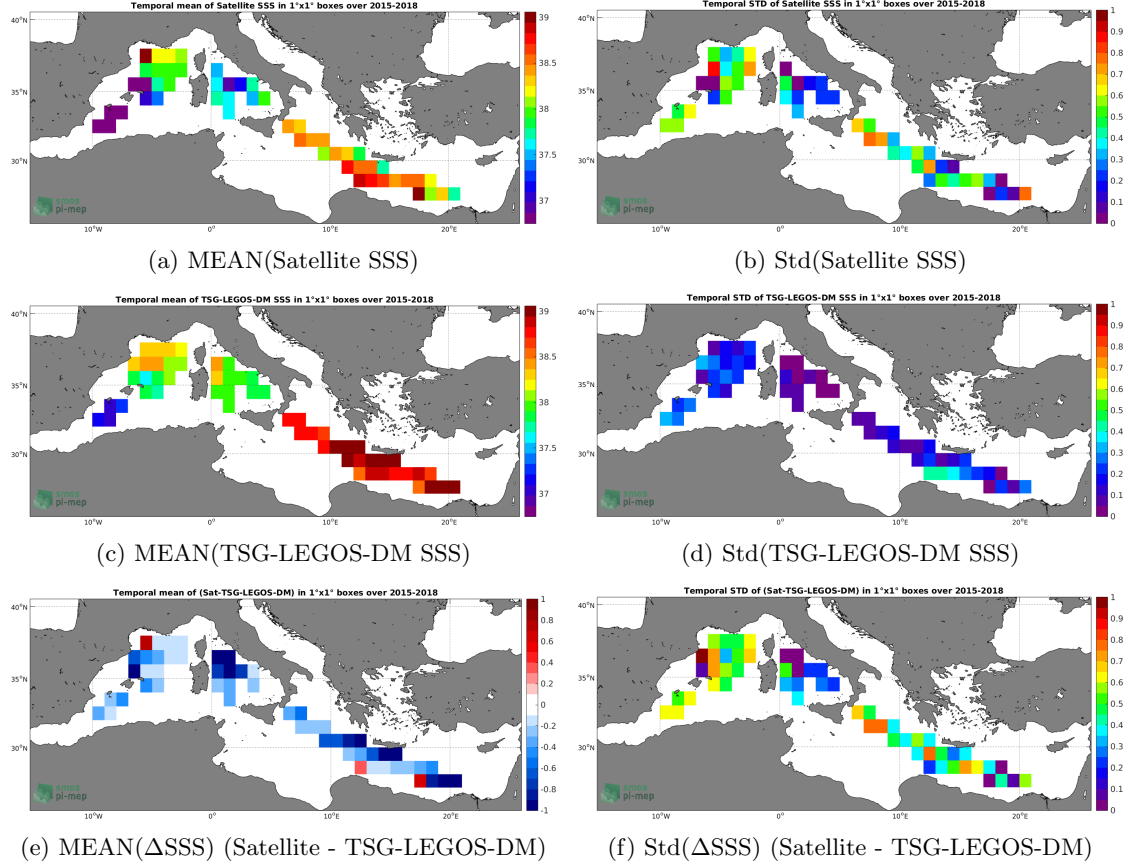
Figure 6: Temporal mean (left) and Std (right) of SSS from SMAP-L2-RSS-V3-70KM (top), TSG-LEGOS-DM (middle), and of \Delta SSS (Satellite - TSG-LEGOS-DM). Only match-up pairs are used to generate these maps.
