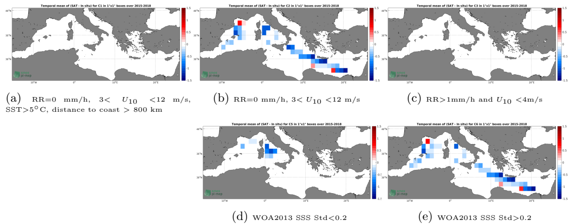
Figure 12: Temporal mean gridded over spatial boxes of size 1^\circ \times 1^\circ of \Delta SSS (SMAP-L2-RSS-V3-70KM - TSG-LEGOS-DM) for 5 different subdatasets corresponding to:RR=0 mm/h, 3 < U_{10} < 12 m/s, SST >5^\circ\text{C} , distance to coast > 800 km (a), RR=0 mm/h, 3 < U_{10} < 12 m/s (b), RR >1 mm/h and U_{10} < 4 m/s (c), WOA2013 SSS Std <0.2 (d), WOA2013 SSS Std >0.2 (e).
