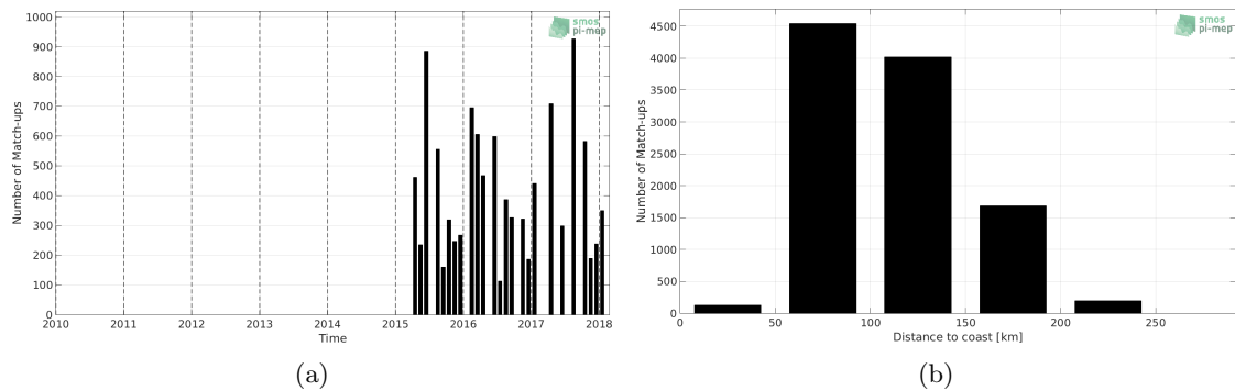
Figure 1: Number of match-ups between TSG-LEGOS-DM and SMAP-L2-RSS-V3-70KM SSS as a function of time (a) and as function of the distance to coast (b) over the Mediterranean Sea Pi-MEP region and for the full satellite product period.
