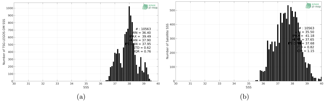
Figure 2: Histograms of SSS from TSG-LEGOS-DM (a) and SMAP-L2-RSS-V3-70KM (b) considering all match-up pairs per bins of 0.1 over the Mediterranean Sea Pi-MEP region and for the full satellite product period.
