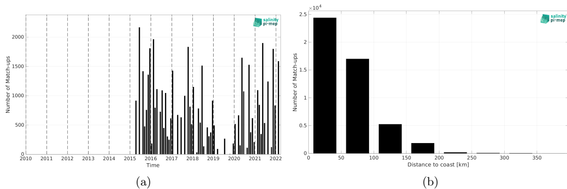
Figure 2: Number of match-ups between TSG (LEGOS-DM) and SMAP SSS L2 v5.0 (JPL) SSS as a function of time (a) and as function of the distance to coast (b) over the Mediterranean Sea Pi-MEP region and for the full satellite product period.
