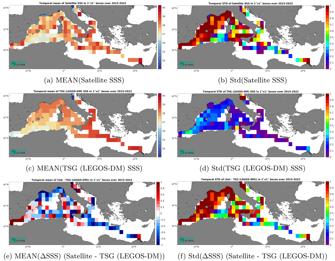
Figure 7: Temporal mean (left) and Std (right) of SSS from SMAP SSS L2 v5.0 (JPL) (top), TSG (LEGOS-DM) (middle), and of \Delta SSS (Satellite - TSG (LEGOS-DM)). Only match-up pairs are used to generate these maps.
