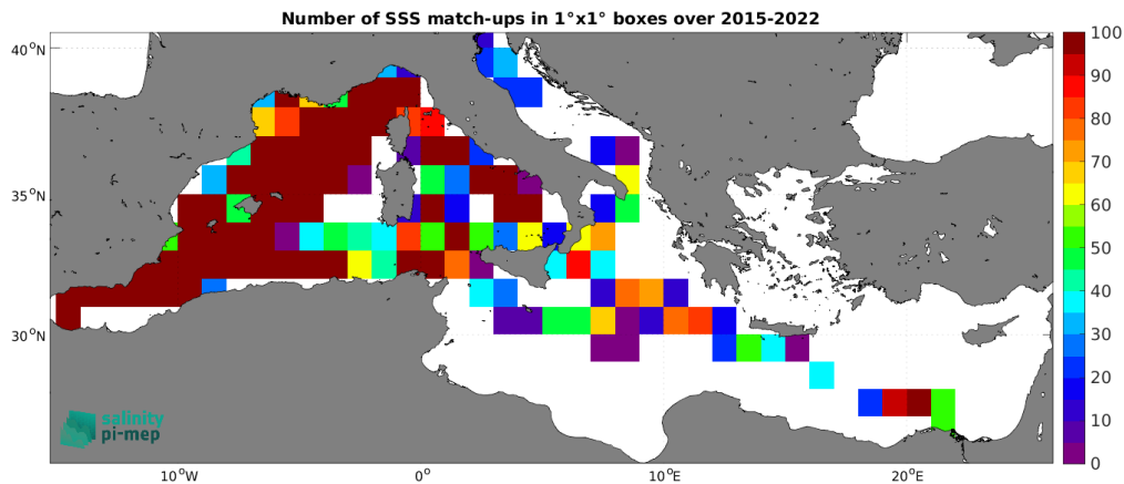
Figure 5: Number of SSS match-ups between TSG (LEGOS-DM) SSS and the SMAP SSS L2 v5.0 (JPL) SSS product for the Mediterranean Sea Pi-MEP region over 1^\circ \times 1^\circ boxes and for the full satellite product period.
