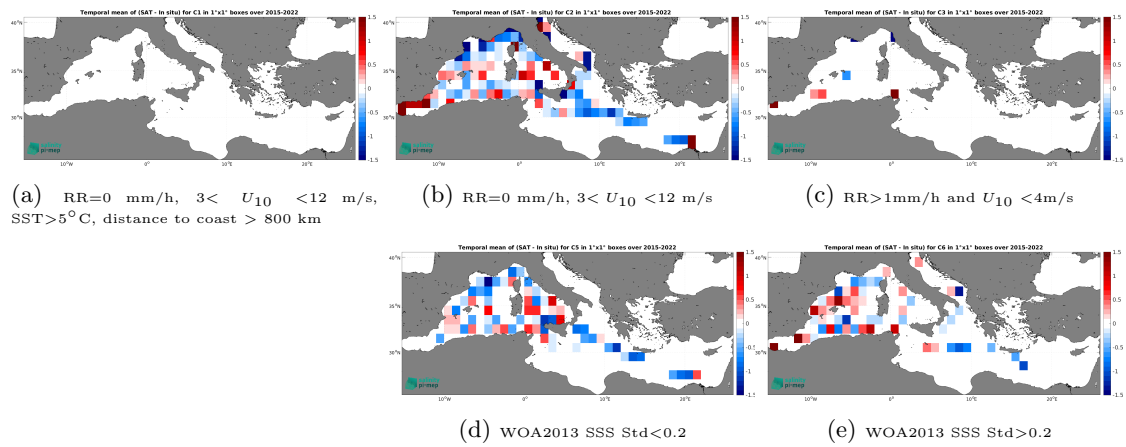
Figure 14: Temporal mean gridded over spatial boxes of size 1^\circ \times 1^\circ of \Delta SSS (SMAP SSS L2 v5.0 (JPL) - TSG (LEGOS-DM)) for 5 different subdatasets corresponding to:RR=0 mm/h, 3 < U_{10} < 12 m/s, SST>5°C, distance to coast > 800 km (a), RR=0 mm/h, 3 < U_{10} < 12 m/s (b), RR>1mm/h and U_{10} < 4 m/s (c), WOA2013 SSS Std<0.2 (d), WOA2013 SSS Std>0.2 (e).
