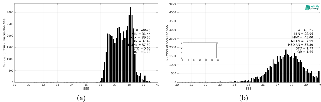
Figure 3: Histograms of SSS from TSG (LEGOS-DM) (a) and SMAP SSS L2 v5.0 (JPL) (b) considering all match-up pairs per bins of 0.1 over the Mediterranean Sea Pi-MEP region and for the full satellite product period.
