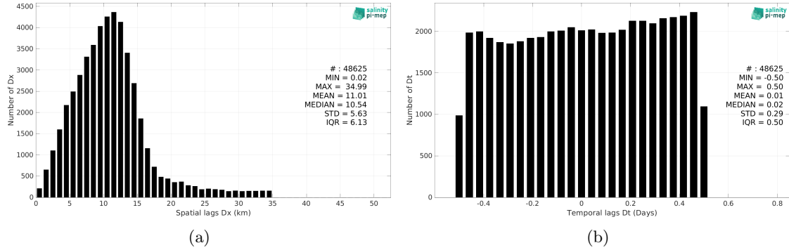
Figure 6: Histograms of the spatial (a) and temporal (b) lags between the location/time of the TSG (LEGOS-DM) measurement and the date of the corresponding SMAP SSS L2 v5.0 (JPL) SSS pixel.
