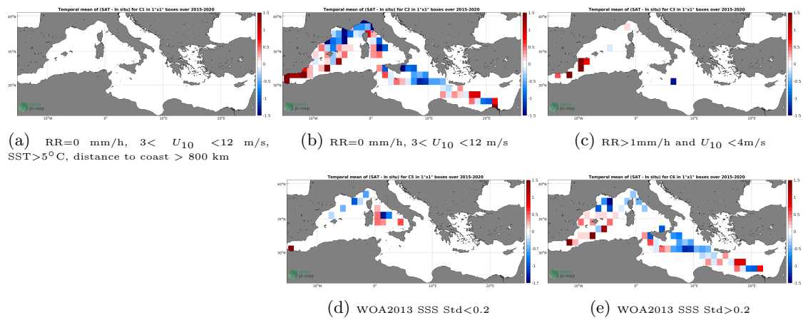
Figure 12: Temporal mean gridded over spatial boxes of size 1^\circ \times 1^\circ of \Delta SSS (SMAP SSS L2 v5.0 (JPL) - TSG (LEGOS-DM)) for 5 different subdatasets corresponding to: RR=0 mm/h, 3 < U_{10} < 12 m/s, SST > 5°C, distance to coast > 800 km (a), RR=0 mm/h, 3 < U_{10} < 12 m/s (b), RR > 1mm/h and U_{10} < 4 m/s (c), WOA2013 SSS Std < 0.2 (d), WOA2013 SSS Std > 0.2 (e).
