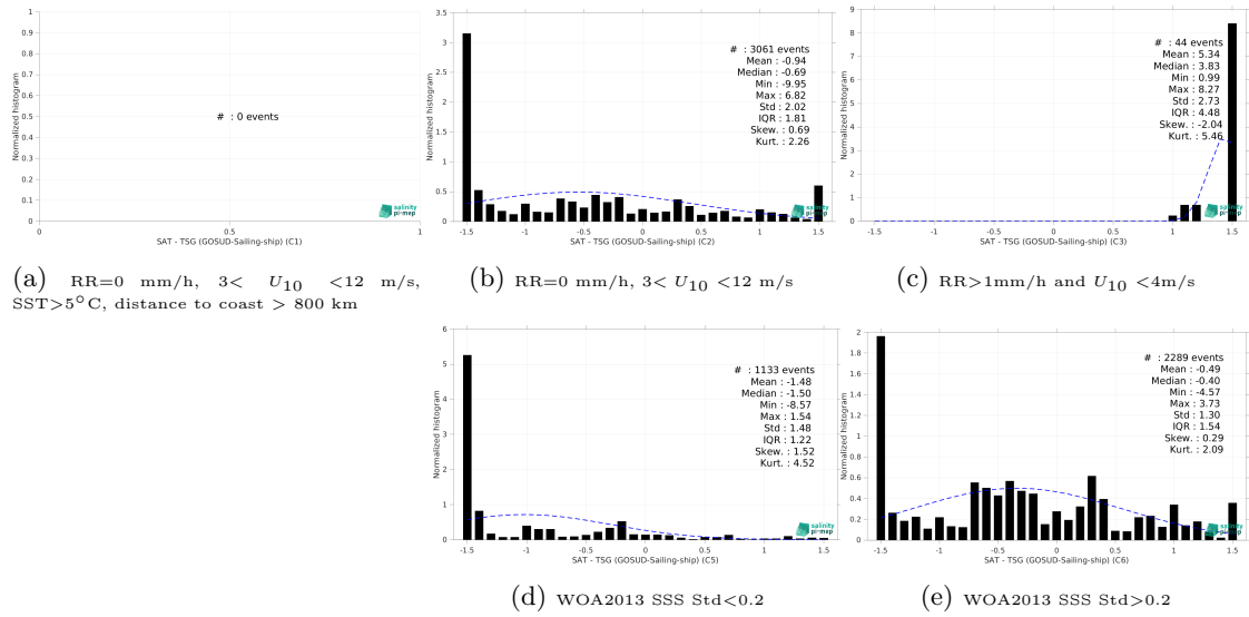
Figure 15: Normalized histogram of \Delta\text{SSS} (SMAP SSS L2 v5.0 (JPL) - TSG (GOSUD-Sailing-ship)) for 5 different subdatasets corresponding to: RR=0 mm/h, 3 < U_{10} < 12 m/s, SST > 5^\circ\text{C} , distance to coast > 800 km (a), RR=0 mm/h, 3 < U_{10} < 12 m/s (b), RR > 1\text{mm/h} and U_{10} < 4\text{m/s} (c), WOA2013 SSS \text{Std} < 0.2 (d), WOA2013 SSS \text{Std} > 0.2 (e).
