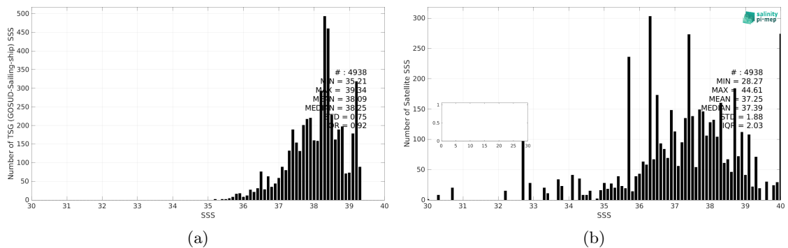
Figure 3: Histograms of SSS from TSG (GOSUD-Sailing-ship) (a) and SMAP SSS L2 v5.0 (JPL) (b) considering all match-up pairs per bins of 0.1 over the Mediterranean Sea Pi-MEP region and for the full satellite product period.
