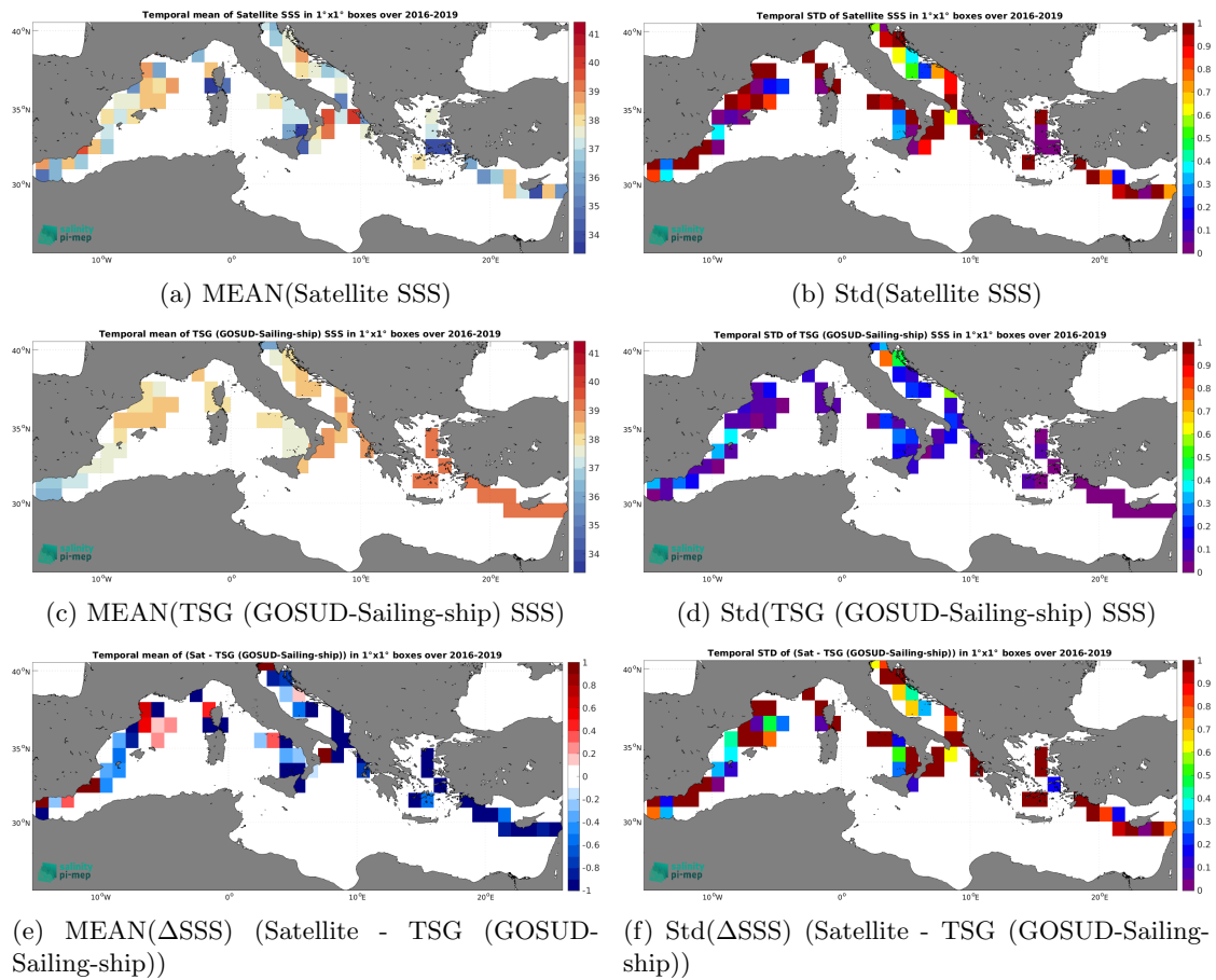
Figure 7: Temporal mean (left) and Std (right) of SSS from SMAP SSS L2 v5.0 (JPL) (top), TSG (GOSUD-Sailing-ship) (middle), and of \Delta SSS (Satellite - TSG (GOSUD-Sailing-ship)). Only match-up pairs are used to generate these maps.
