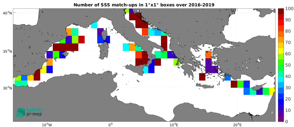
Figure 5: Number of SSS match-ups between TSG (GOSUD-Sailing-ship) SSS and the SMAP SSS L2 v5.0 (JPL) SSS product for the Mediterranean Sea Pi-MEP region over 1^\circ \times 1^\circ boxes and for the full satellite product period.
