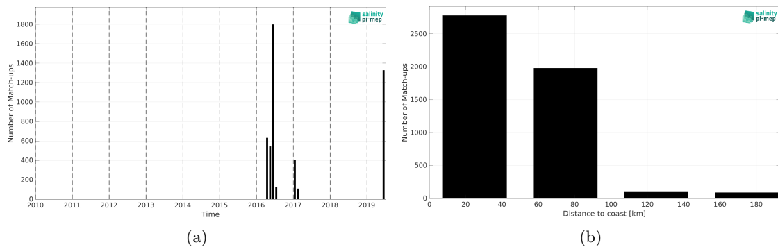
Figure 2: Number of match-ups between TSG (GOSUD-Sailing-ship) and SMAP SSS L2 v5.0 (JPL) SSS as a function of time (a) and as function of the distance to coast (b) over the Mediterranean Sea Pi-MEP region and for the full satellite product period.
