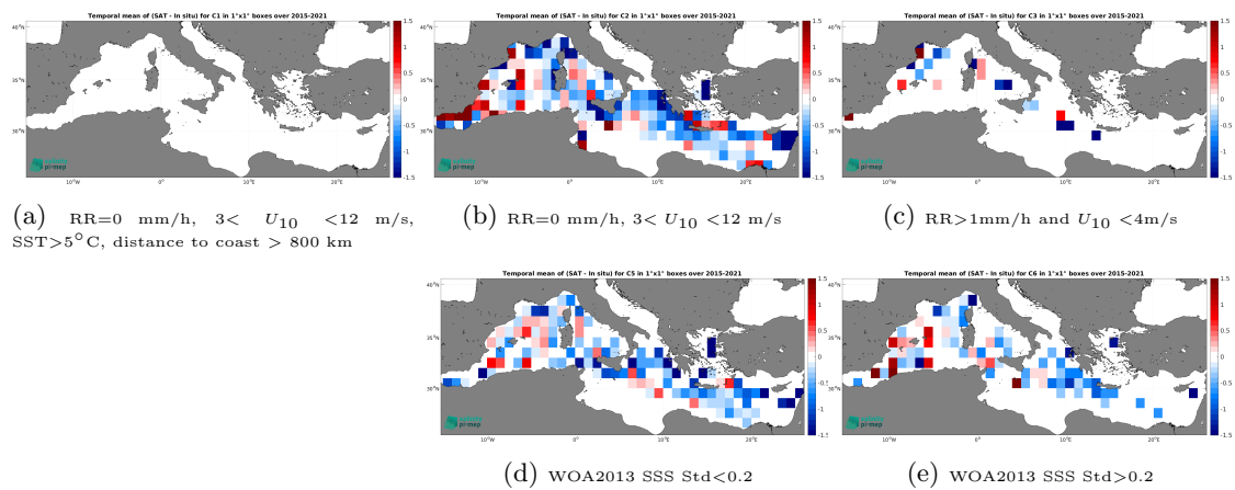
Figure 12: Temporal mean gridded over spatial boxes of size 1^\circ \times 1^\circ of \Delta\text{SSS} (SMAP SSS L2 v5.0 (JPL) - TSG (GOSUD-Research-vessel)) for 5 different subdatasets corresponding to:RR=0 mm/h, 3 < U_{10} < 12 m/s, SST >5^\circ\text{C} , distance to coast > 800 km (a), RR=0 mm/h, 3 < U_{10} < 12 m/s (b), RR >1 mm/h and U_{10} < 4 m/s (c), WOA2013 SSS Std <0.2 (d), WOA2013 SSS Std >0.2 (e).
