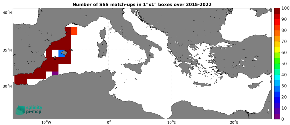
Figure 4: Number of SSS match-ups between TSG (CSIC-UTM) SSS and the SMAP SSS L2 v5.0 (JPL) SSS product for the Mediterranean Sea Pi-MEP region over 1^\circ \times 1^\circ boxes and for the full satellite product period.
