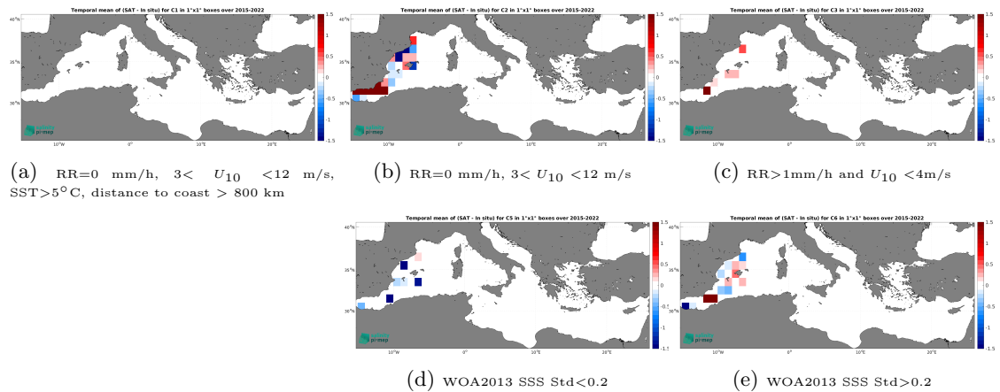
Figure 12: Temporal mean gridded over spatial boxes of size 1^\circ \times 1^\circ of \Delta SSS (SMAP SSS L2 v5.0 (JPL) - TSG (CSIC-UTM)) for 5 different subdatasets corresponding to:RR=0 mm/h, 3 < U_{10} < 12 m/s, SST >5^\circ\text{C} , distance to coast > 800 km (a), RR=0 mm/h, 3 < U_{10} < 12 m/s (b), RR >1 mm/h and U_{10} < 4 m/s (c), WOA2013 SSS Std <0.2 (d), WOA2013 SSS Std >0.2 (e).
