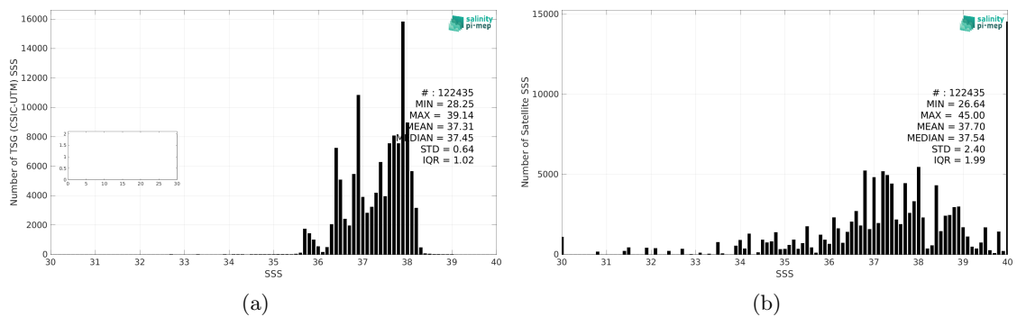
Figure 2: Histograms of SSS from TSG (CSIC-UTM) (a) and SMAP SSS L2 v5.0 (JPL) (b) considering all match-up pairs per bins of 0.1 over the Mediterranean Sea Pi-MEP region and for the full satellite product period.
