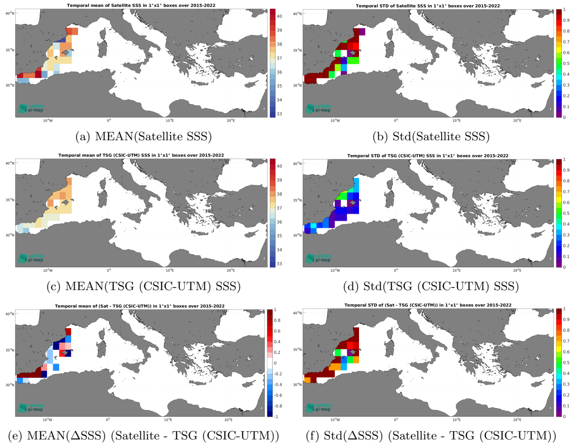
Figure 6: Temporal mean (left) and Std (right) of SSS from SMAP SSS L2 v5.0 (JPL) (top), TSG (CSIC-UTM) (middle), and of \Delta SSS (Satellite - TSG (CSIC-UTM)). Only match-up pairs are used to generate these maps.
