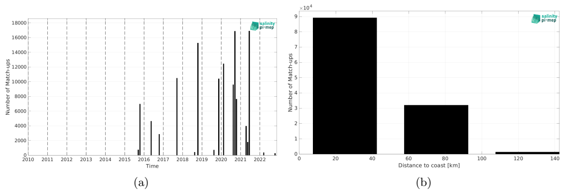
Figure 1: Number of match-ups between TSG (CSIC-UTM) and SMAP SSS L2 v5.0 (JPL) SSS as a function of time (a) and as function of the distance to coast (b) over the Mediterranean Sea Pi-MEP region and for the full satellite product period.
